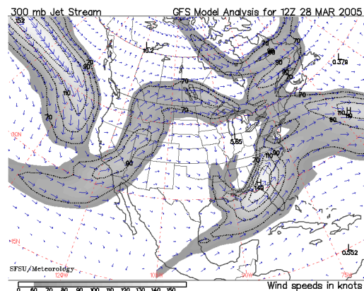
Fig. 2 These two charts show how the position of the jet stream is forced equatorward during an El Niño event. They show two days (27 and 28 MAR 2005) of the jet stream. The trough is pushed south of Florida into the Gulf of Mexico. Taken from http://squall.sfsu.edu/crws/jetstream.html on 28MAR05.
