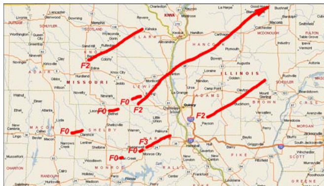
Fig 1. Map of tornado tracks (F-scale denoted) within the LSX CWA in northeast Missouri and west central Illinois.
