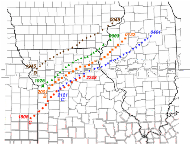
Fig 2. Plot of the maximum radar reflectivity centroid tracks of selected supercells (annotated A-D). The first point is the initial cell with subsequent positions every 15 minutes. Annotated times are UTC.
