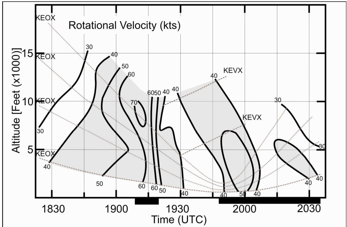
Figure 6. Time-height of rotational velocity of the Enterprise and Echo, Alabama mesocyclones on 1 March 2007 constructed from velocity scans from the KEOX and KEVX WSR-88D radars..
