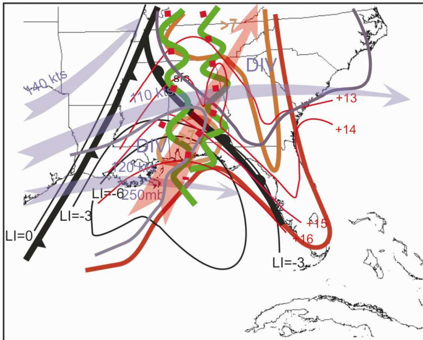
Figure 3. Composite chart for 1800 UTC, 1 March 2007.
