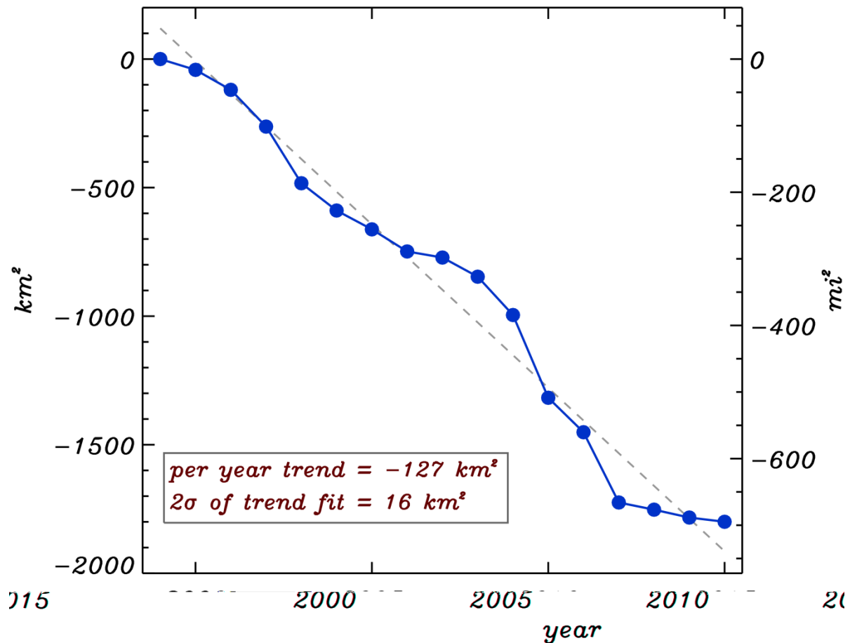
Fig. 3.5. Cumulative net area change (km 2 and square miles, left and right axes, respectively) at the 45 of the widest and fastest-flowing marine-terminating glaciers of the Greenland Ice Sheet (after Box and Decker 2011 and Jensen et al. unpublished). The linear regression is dashed.
