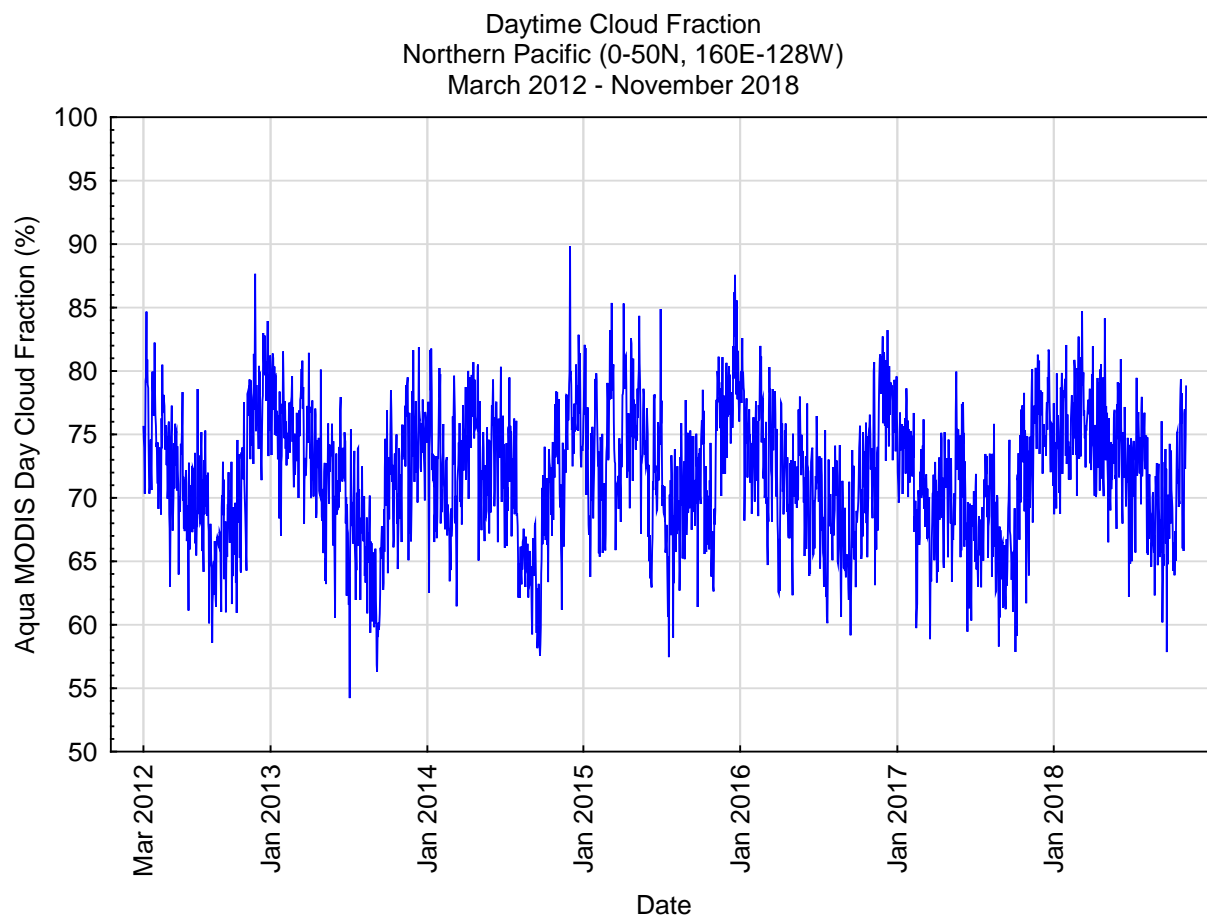
Figure 2. Time series of daily mean cloud fractions taken from MVCM Aqua MODIS pixel-level results.
