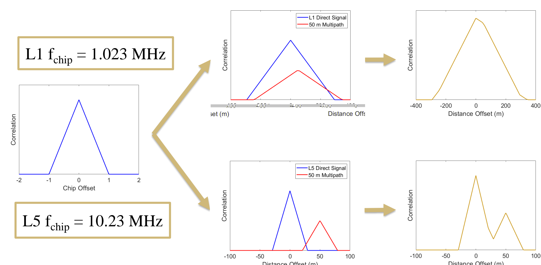
Figure 2. Comparison of GPS signal correlation peak for GPS L1 and L5 signals. Notably, the L5 correlation has a much higher precision and can easily be distinguished from a 50 m multipath error, while the L1 signal is degraded by multipathing.
