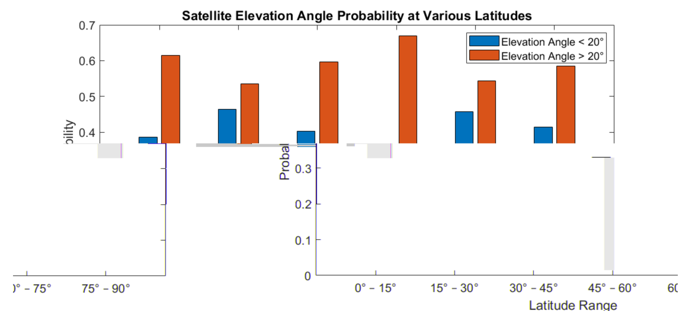
Figure 1. Probability of received narrowband GPS signals below and above 20° satellite elevation angle binned by latitude range.
