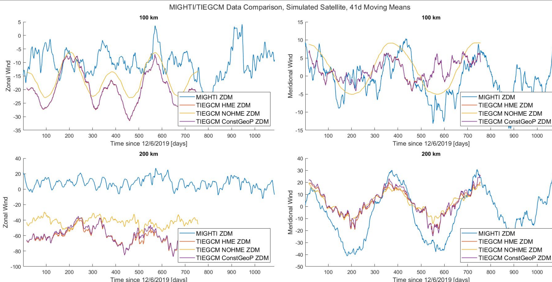
Figure 1: Time series of binned MIGHTI ZDMs compared with equivalently binned TIEGCM model output ZDMs using Hough Mode Extension boundary conditions & space weather parameterization on/off.
