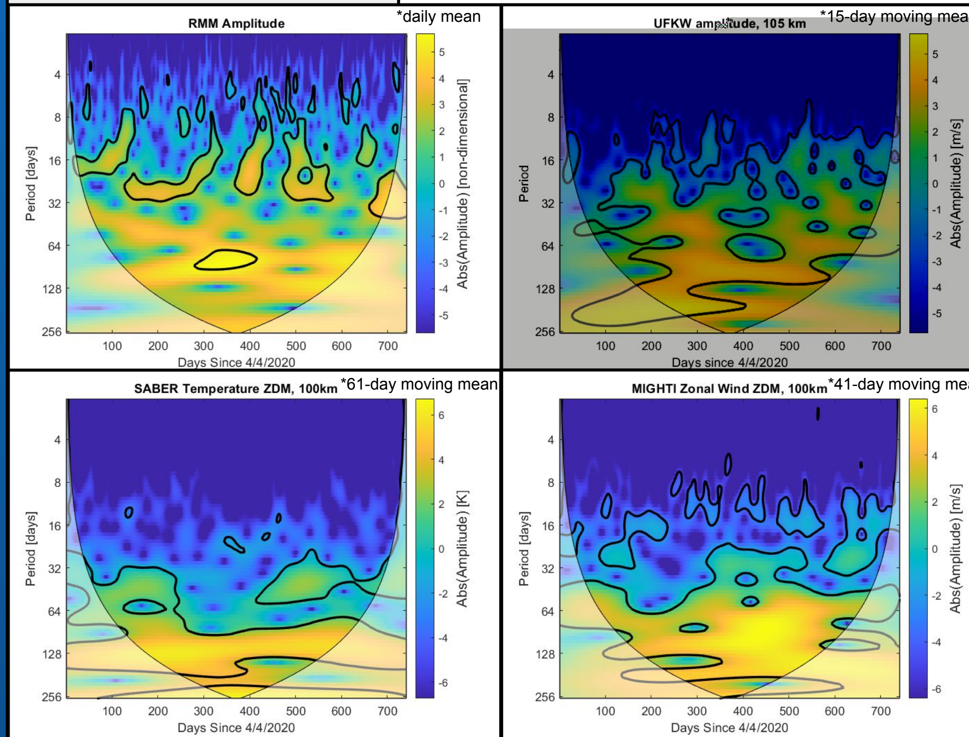
Figure 6: Morlet wavelet scalograms of RMM amplitude, UFKW amplitude, SABER temperatures, and MIGHTI zonal wind ZDMs at 100 km. 95% confidence contours.
