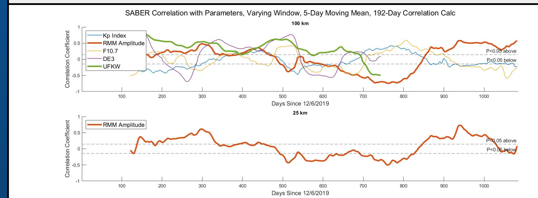
Figure 4: Correlation between SABER temperatures and Kp index, RMM amplitude, F10.7, UFKWs, and DE3 tides at 25 km and 100 km. Statistically significant data outside dashed lines
