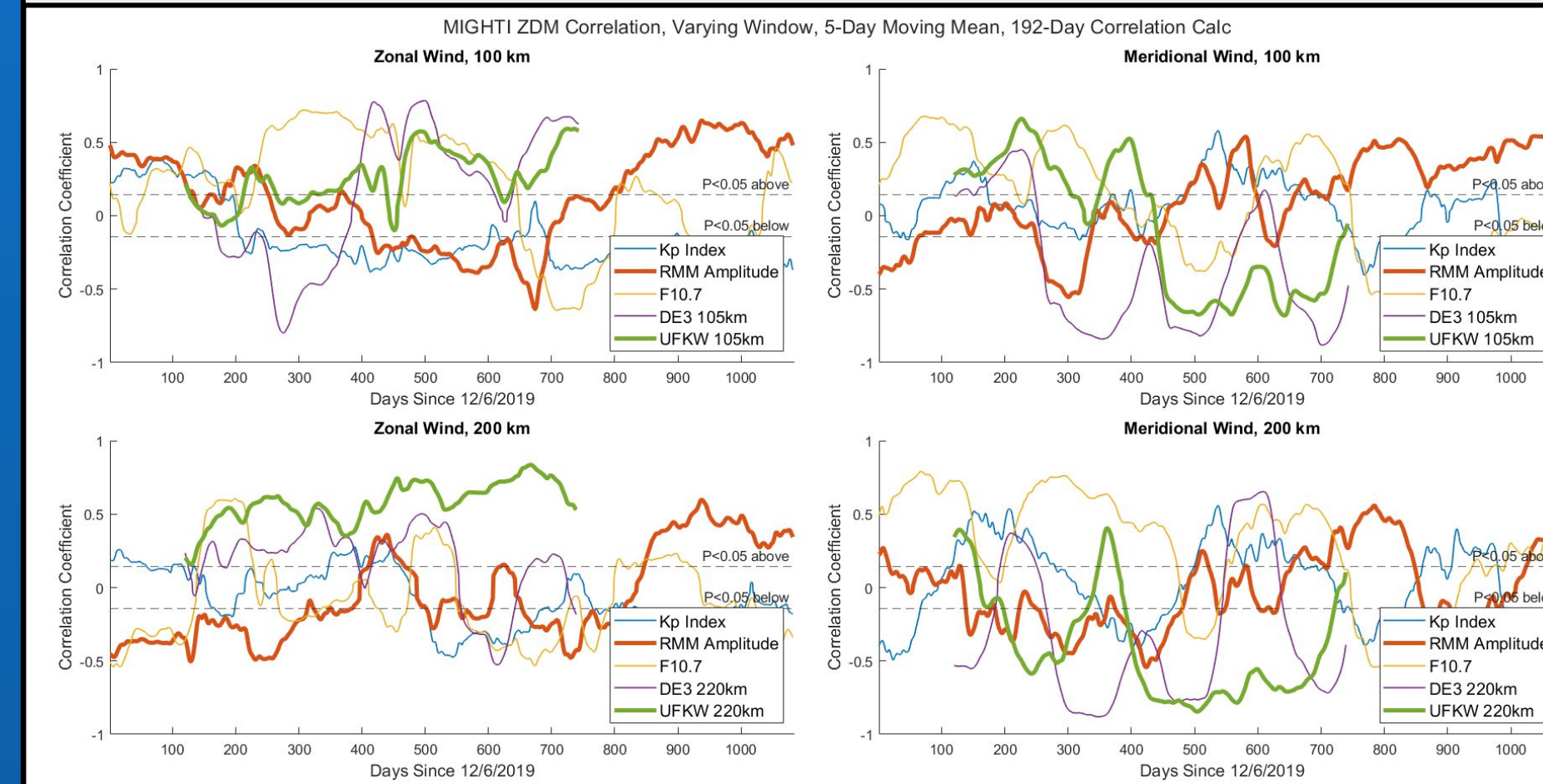
Figure 2: Correlation between MIGHTI zonal diurnal mean wind components and Kp index, RMM amplitude, F10.7, DE3 tides, and UFKW at 100 km and 200 km MSL. Statistically significant data outside dashed lines.
