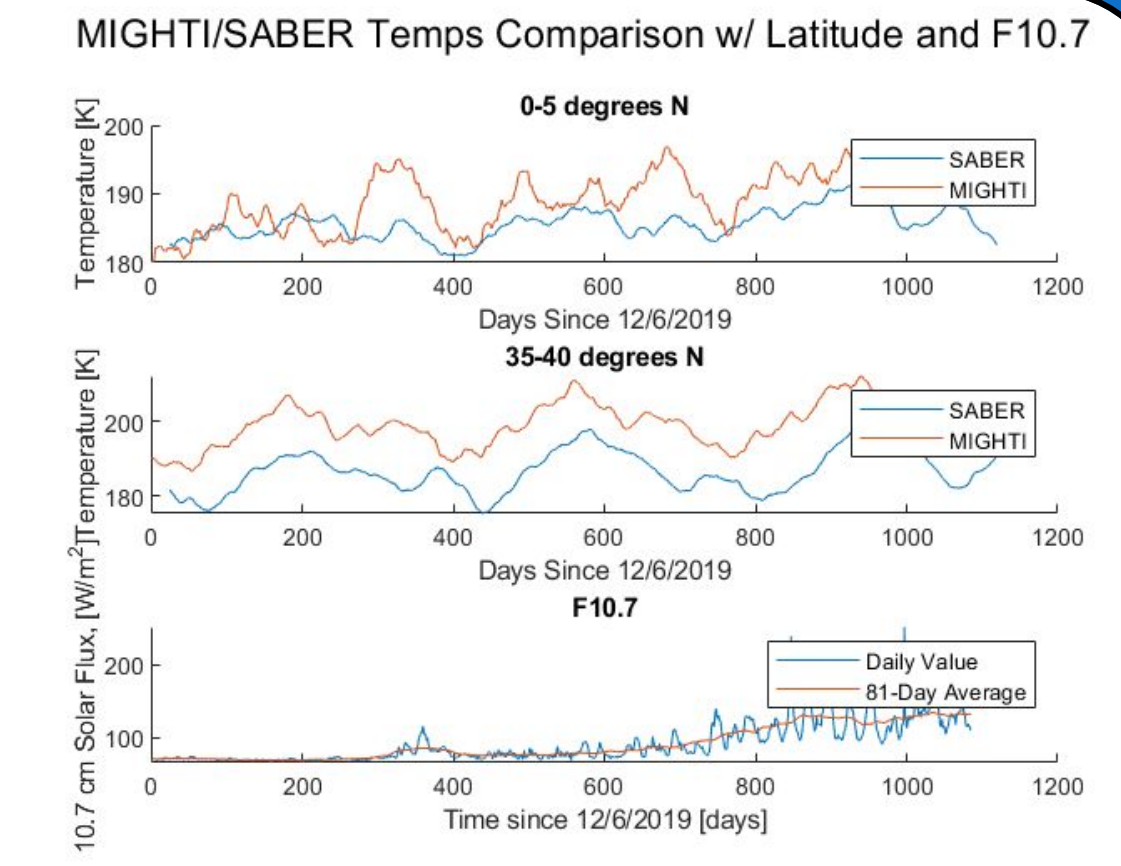
Figure 5: Comparison of MIGHTI and SABER ZDM temperatures at the equator and the mid-latitudes alongside F10.7.
