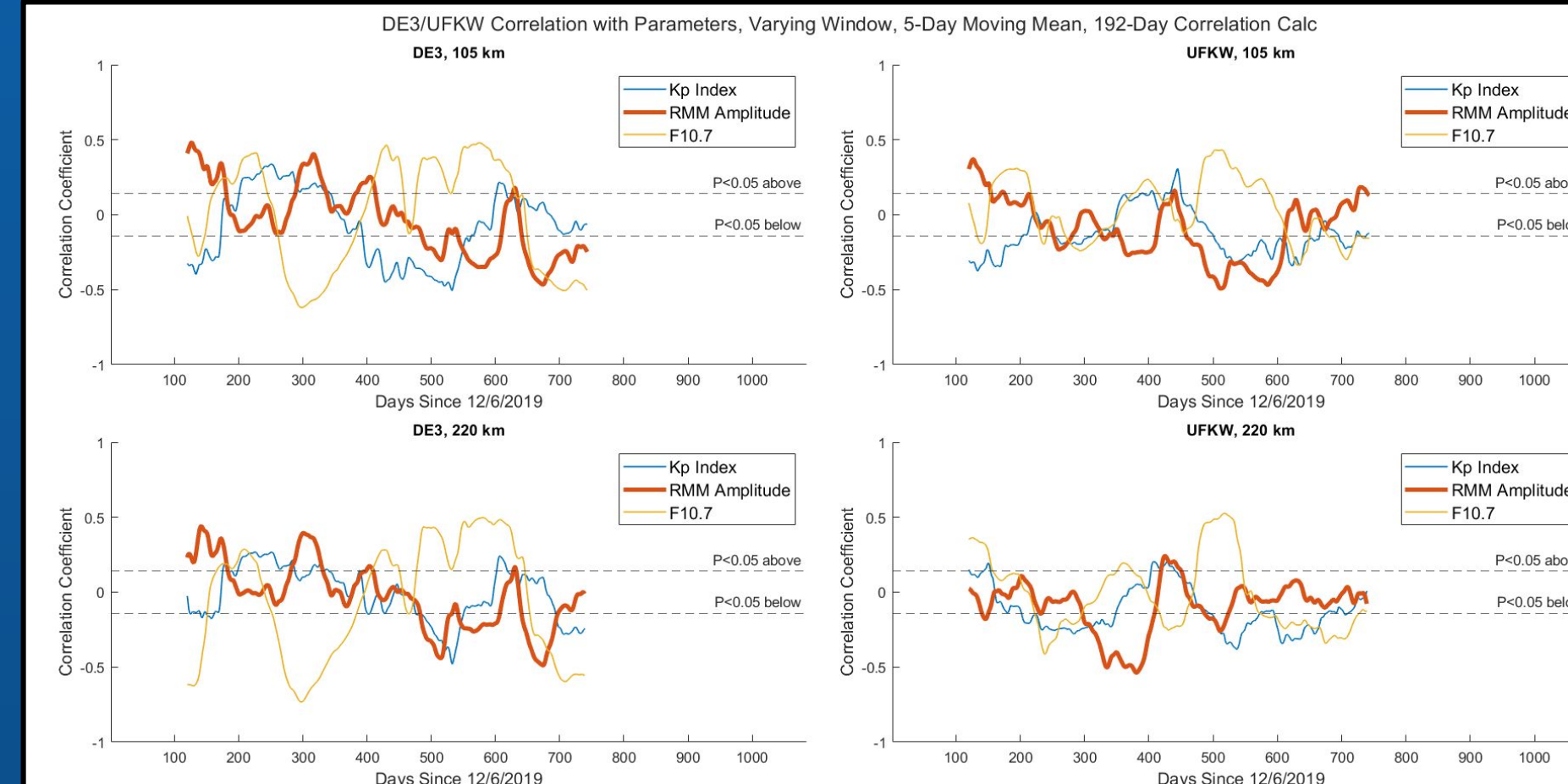
Figure 3: Correlation between DE3 tides/UFKW and Kp index, RMM amplitude, and F10.7. Statistically significant data outside dashed lines.
