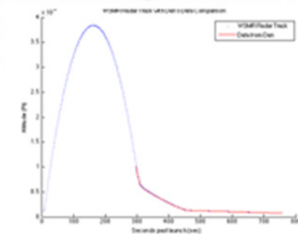
ADS-B data aligned with radar data
