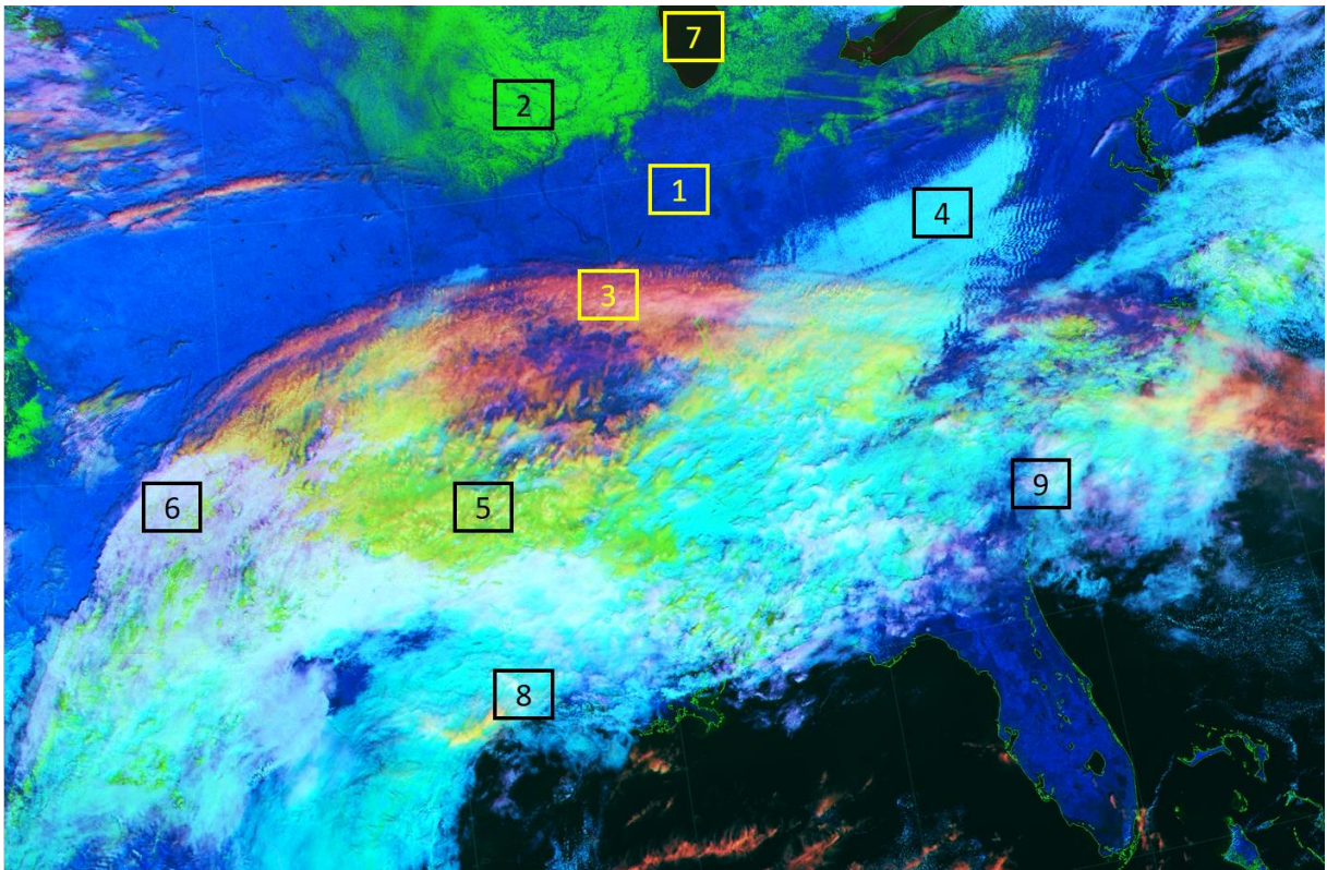
Figure 6.4. RGB Cloud Types product from GOES-16 satellite.
