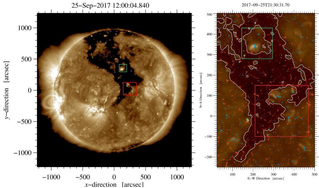
Figure 2.12. Left: AIA EUV 193 Å images of non-polar coronal hole on 25 September 2017. The green and red boxes refer to regions of interest studied in detail. The coronal hole boundary is outlined by white contours (right). Positive and negative polarities derived from HMI magnetograms are displayed in red and blue, respectively.
