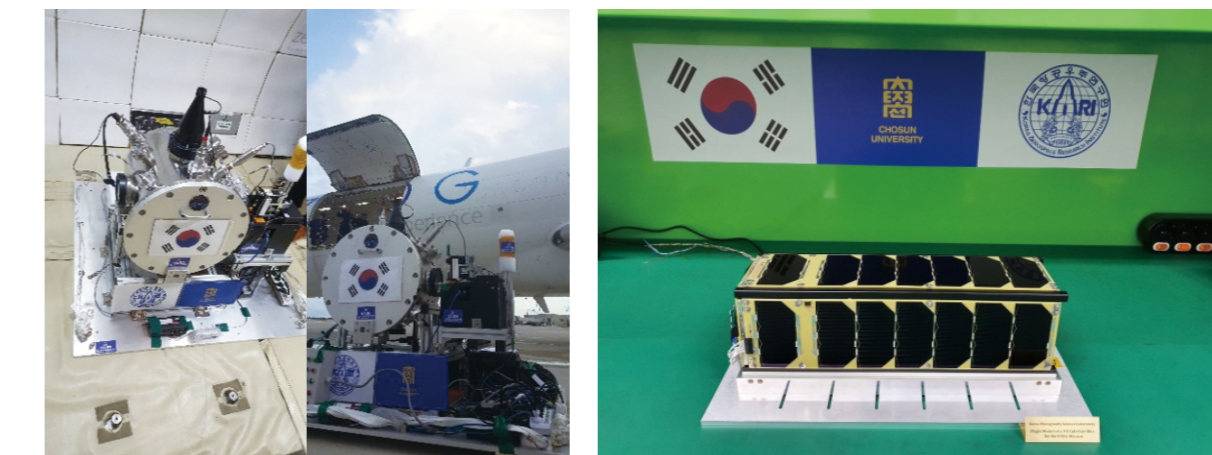
Figure 1. Combustion chamber and auxiliary devices (left) Figure 2. Flight Model of the KMSL nanosatellite (right)
