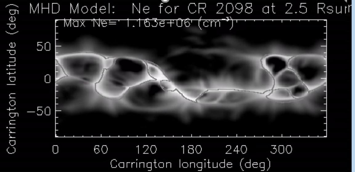
MHD model by PSI
