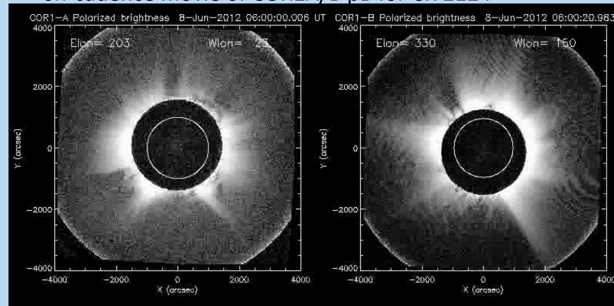
6h-cadence movie of COR1A/B pB for CR 2124
