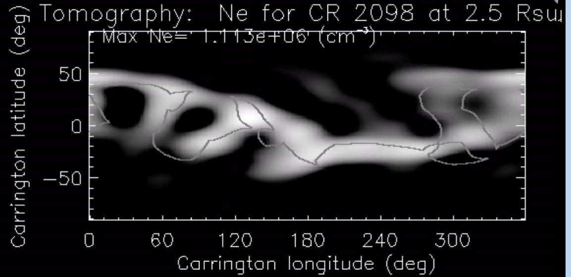
Regularization with a weighting factor
