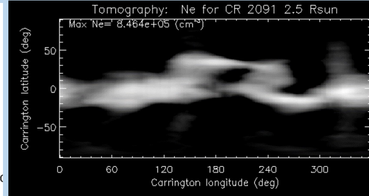
Tomographic density reconstructed from the same pB observations
