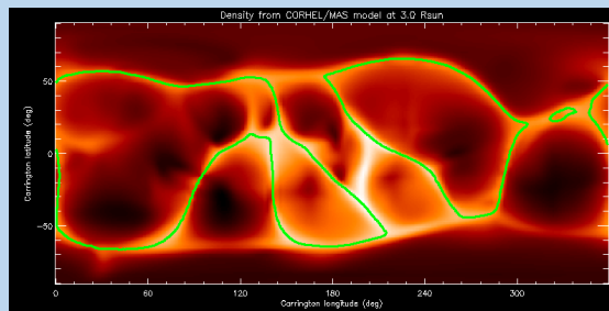
PSI MHD steady-state N at r=3 R_s (green contours for B_r=0 )
