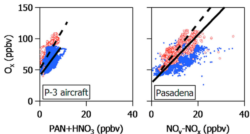
Figure P4. Plots of (left) airborne observations of O_x versus PAN+HNO_3 and (right) ground-based measurements of O_x versus NO_y-NO_x on weekdays (blue dots, solid lines) and weekends (red circles, dashed lines). (Figure from Pollack et al. , 2012).
