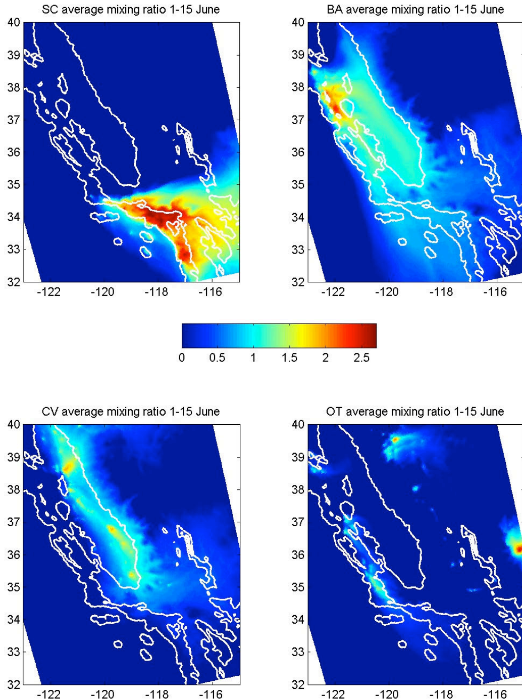
Figure R1: Average near-surface mixing ratios of each CO tracer (log 10 (ppbv)) for all hours of 1-15 June, 2010. Log (base 10) scale is used to make small concentrations visible. The maps span from the Sacramento Valley in the northwest to the California-Mexico border in the southeast; the white lines show the 1 m and 500 m elevation contours. In the model calculation, a background CO concentration of 120 ppbv is assumed, but that background is not added in this figure. The tracers are identified according to their emission region: Southern California (SC), San Francisco Bay Area (BA), Central Valley (CV) and other regions (OT). [Figure from Angevine et al. , 2013].
