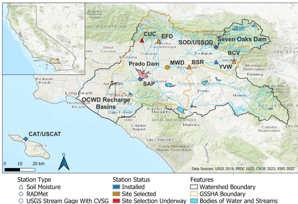
Figure 6-2. The Prado FIRO Observation Network.
