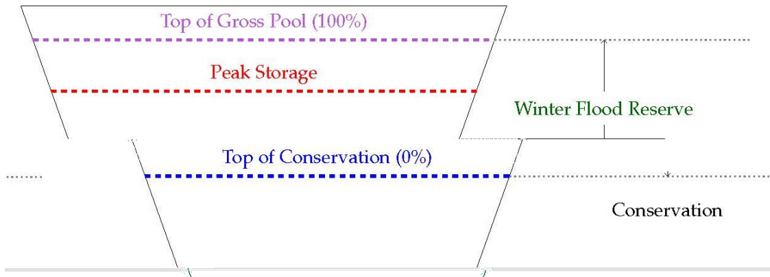
Figure I-1. Reservoir Utilization Risk Metric Diagram
