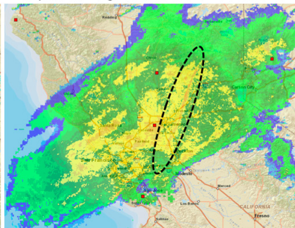
Example of Convergence at 0045 UTC 25 October 2021
