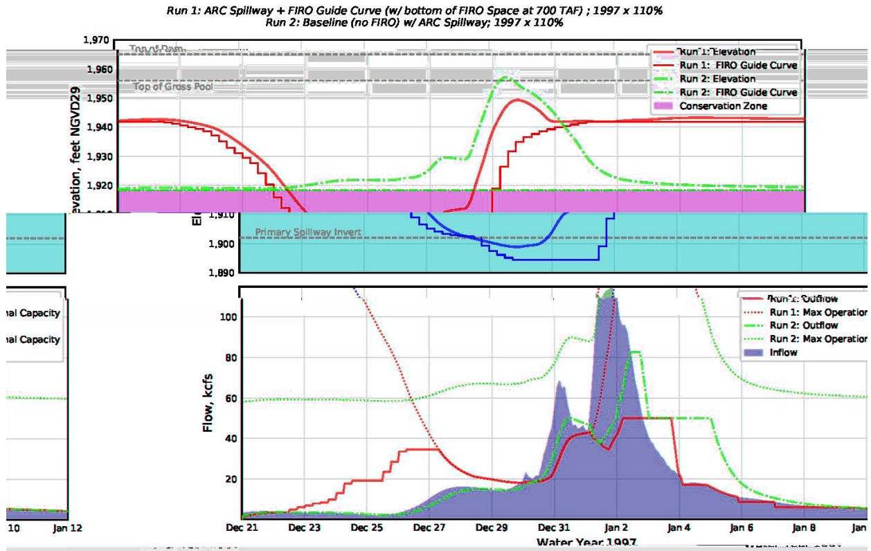
Figure E-6. Comparison between Operations with Baseline (no FIRO) and Candidate Guide Curve; 1997 110%
