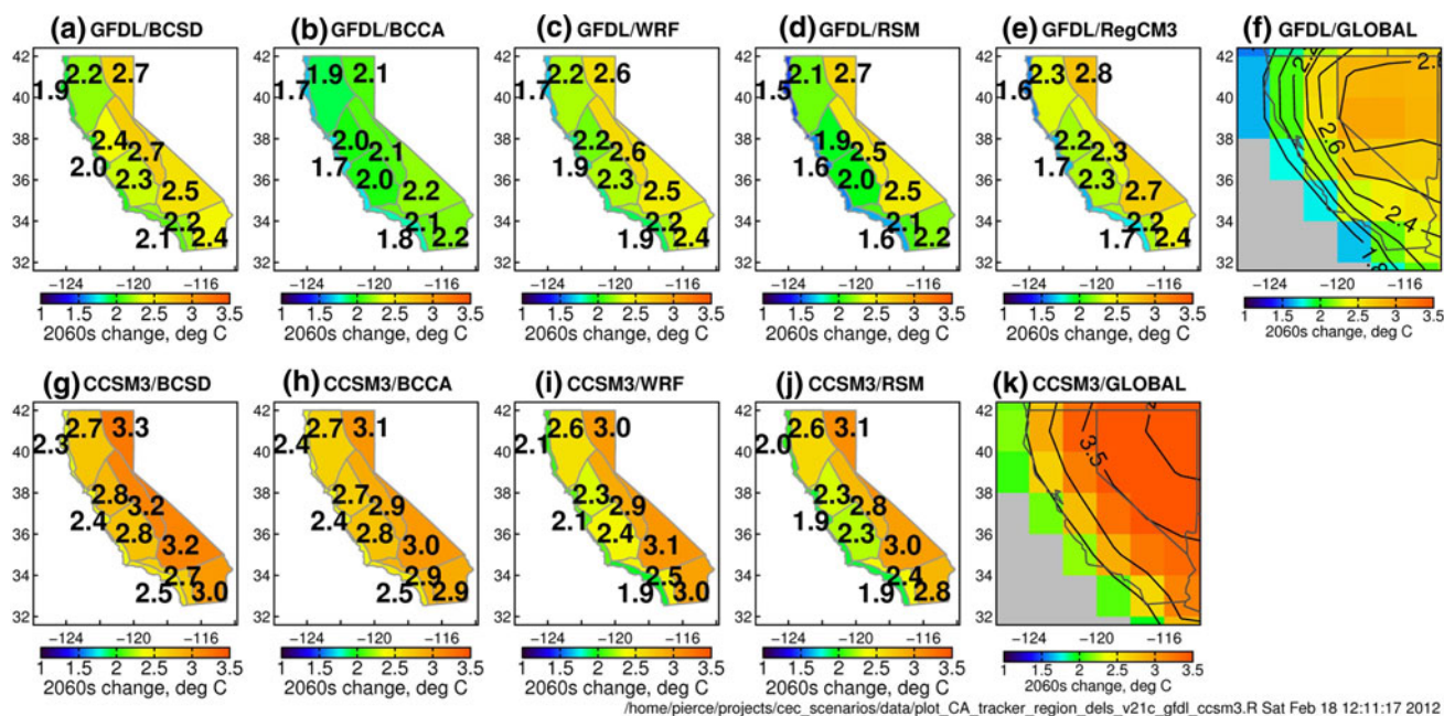
Fig. 3 Yearly temperature change ( ^{\circ}\text{C} ) (2060–2069 minus 1985–1994) from each downscaling technique applied to the GFDL 2.1 global model ( upper ) and CCSM3 global model ( lower ). The yearly temperature changes from the global models are shown in (f) and (k), for comparison
