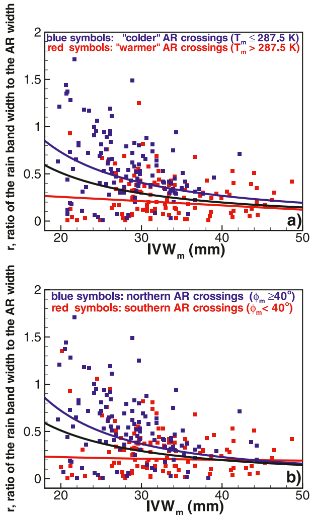
FIG. 4. The ratio of the rainband width to the AR width as a function of the mean value of IWV stratified with respect to the (a) AR temperature near the surface T_m and (b) mean latitude of AR crossings \phi_m . For the entire dataset blue, red, and black curves show mean trends for colder [in (a), T_m \leq 287.5 K] and more northern crossings [in (b), \phi_m \geq 40^\circ ], warmer [in (a), T_m > 287.5 K] and more southern crossings [in (b), \phi_m < 40^\circ ], and all ARs events correspondingly.
