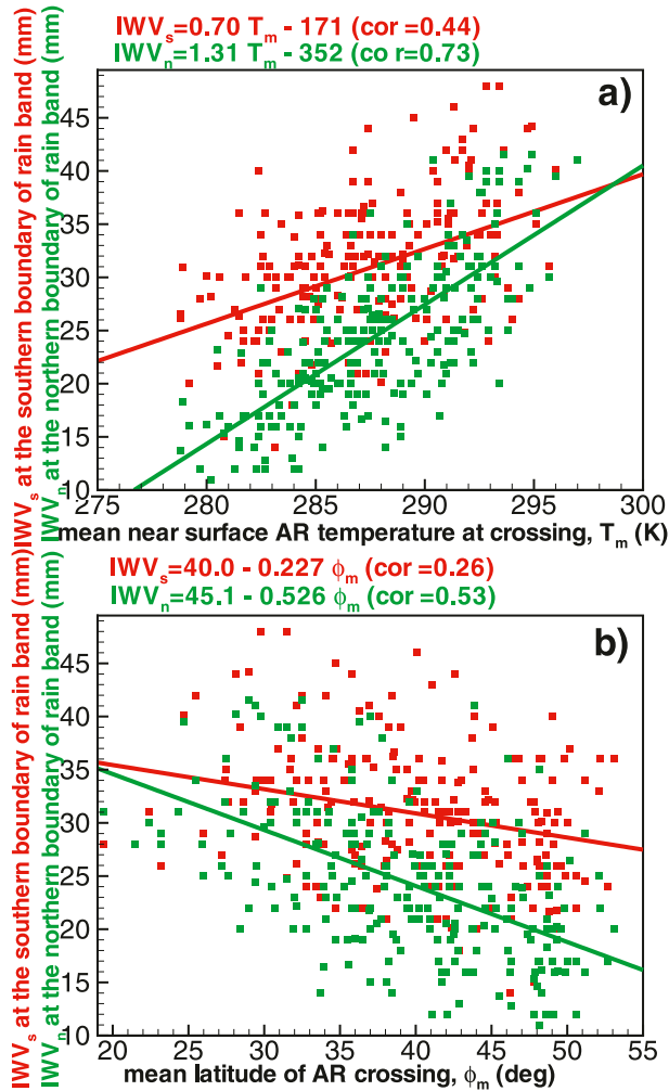
FIG. 6. The scatterplots between IWV at southern ( IWV_s ) and northern ( IWV_n ) boundaries of (a) rainbands associated with AR and AR mean temperature near the surface T_m and (b) a mean latitude of an AR crossing \phi_m , as obtained from the entire 2006 to 2009 dataset.
