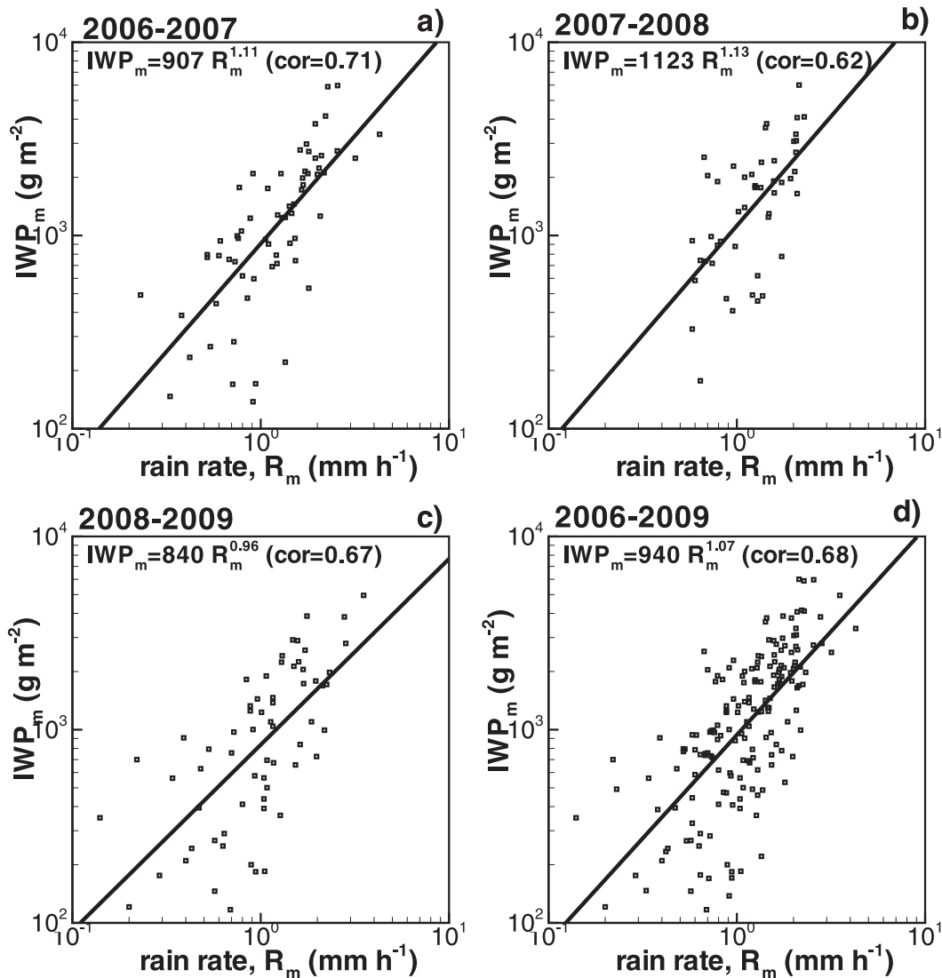
FIG. 7. Scatterplots between mean values of IWP and rain rate retrieved for the regions of cold rain observed at satellite AR crossings during (a) 2006–07, (b) 2007–08, (c) 2008–09, and (d) the entire observational period. Correlation coefficients and best-fit power-law approximations are also shown.
