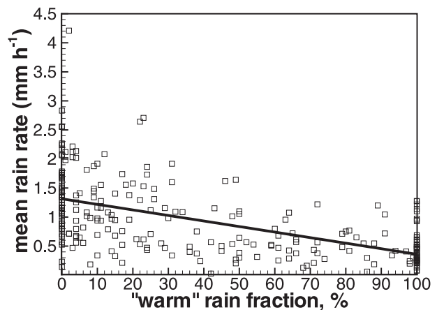
FIG. 3. Mean rain rate as a fraction of warm rain fraction in precipitation observed at AR crossings (2006–09 dataset).
