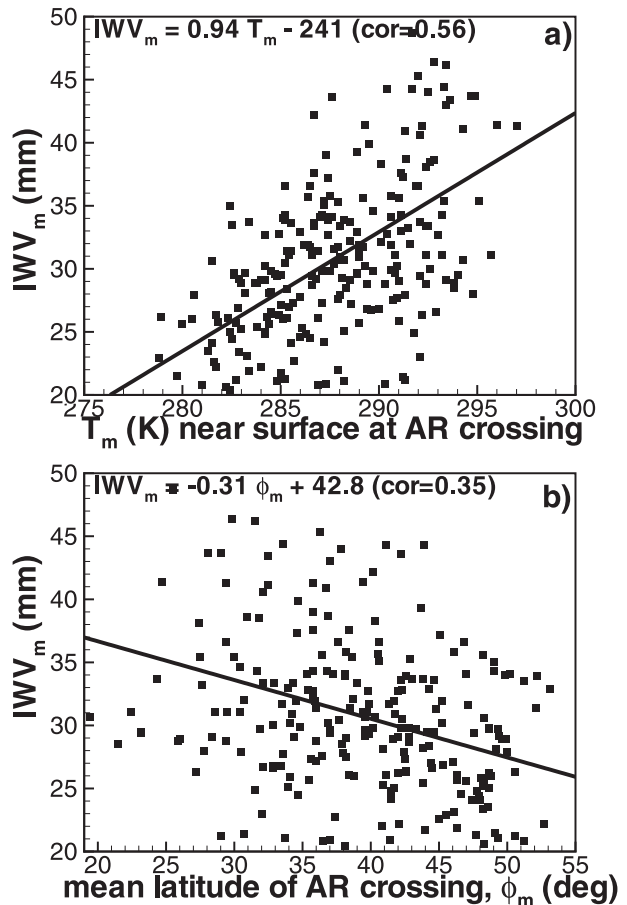
FIG. 5. The scatterplots between IWV_m and (a) the mean AR temperature near the surface T_m and (b) a mean latitude of an AR crossing \phi_m for the entire 2006–09 dataset.
