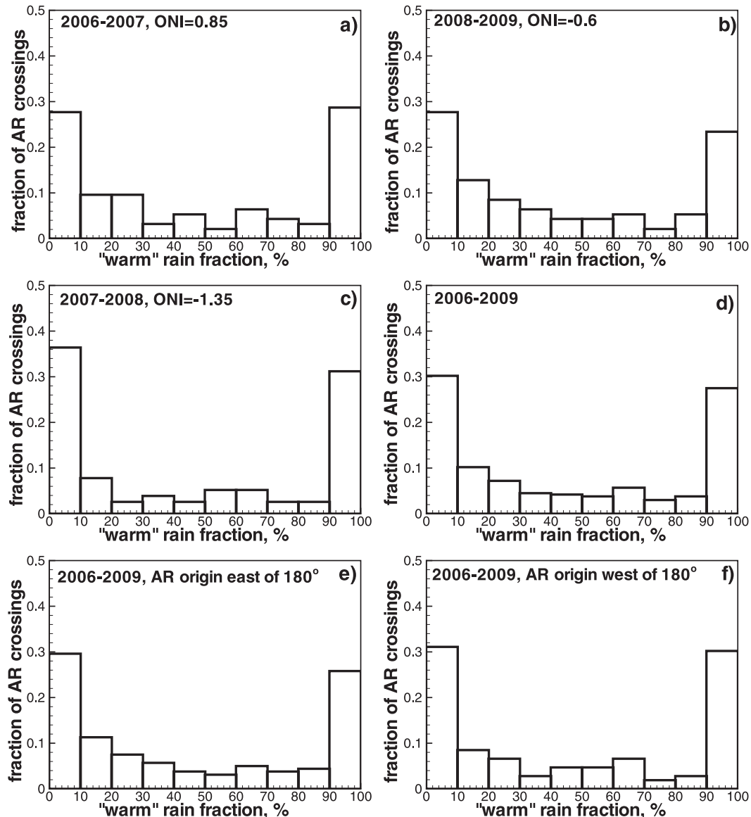
FIG. 2. Histograms of the precipitation regime observed during the satellite AR crossings for the observational (a) 2006–07, (b) 2008–09, and (c) 2007–08 periods, as well as (d) the composite for 2006–09, and the subsets of ARs tapping moisture reservoirs (e) east and (f) west of 180^\circ longitude. The warm rain fraction is defined as the ratio of CPR profiles when the warm rain type is identified to the total number of rain profiles in a crossing.
