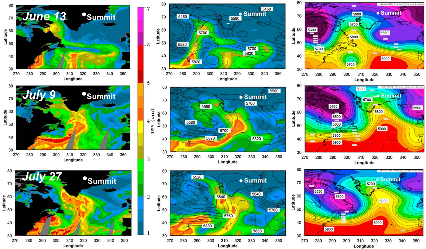
Figure 6. Comparison of (left) SSMI-derived IWV with that from the (middle) Global Forecast System (GFS) analysis and (right) 500 hPa height fields. Scale is the same for both IWV products. Top left: 13 June 12–24Z: The observed and reanalysis-derived IWV show low-total vapor near Greenland. Middle left: 9 July 00–12Z: Strong northward transport, as indicated by the GPH field (right figure), of relatively moist air. Bottom left: 27 July 00–12Z: Strong northward transport of relatively moist air. The observed IWV (left) shows more significant vapor transport to the north along the west coast of Greenland. In all three cases the GFS provides a close approximation, but is slightly drier, compared to the IWV derived from the SSMI. The 500 hPa contours on the right are at 25 m intervals from 5450 m to 5950 m. Note that on the warmest days at Summit the ridge axis intersect the southeast coast of Greenland. On 13 June, the ridge is aligned west of Greenland, and the moisture plume lies largely over land areas. Note that on the second two days the high IWV areas align along the more closely packed contours over the north Atlantic.
