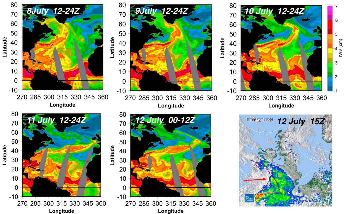
Figure 3. Sequence of SSM/I images (10°S–80°N, 270°E–360°E) following the progression of the AR from when it first impacts Greenland until it makes landfall in France and England (far lower right: http://uk.weather.com/partners-JulyOutlook/71212forecast ). IWV scale at the upper right is from 1 cm to 7 cm). Note the residue IWV left along the west coast Greenland following the AR transition to the east.
