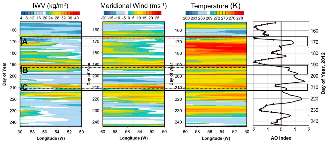
Figure 5. Hovmöller (time-longitude) cross sections of integrated water vapor (IWV, \text{kg/m}^2 ), meridional wind ( \text{ms}^{-1} , 700 hPa), and temperature (K, 700 hPa) for the summer of 2012 just west of Greenland between 50^\circ\text{W} and 60^\circ\text{W} and averaged from 60^\circ\text{N} to 65^\circ\text{N} . Three warming periods (A, B, C) are indicated by the boxed areas and correspond to the periods of maximum temperature at Summit shown in Figure 4. Dashed lines indicate the times of maximum temperatures for each case at Summit which are later than the increases at the west coast. The time series of the Arctic Oscillation (AO) to the right provides a comparison of each event with rapid changes in the state of the AO.
