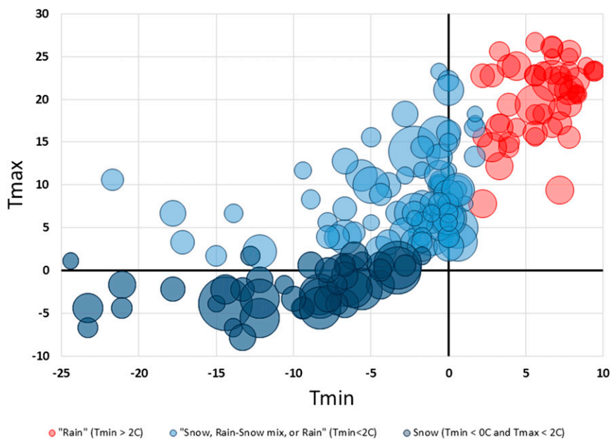
FIG. 5. Min daily temperature ( x axis; ^{\circ}\text{C} ) vs max daily temperature ( y axis; ^{\circ}\text{C} ) for precipitation events occurring above 2500-m elevation. Circle color indicates likely phase (rain, snow, or mixed) of precipitation shaded according to legend. Circle size indicates relative magnitude of 24-h precipitation total per event.
