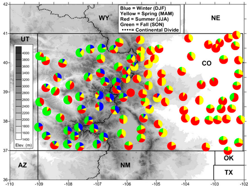
FIG. 2. Seasonality of the top 10 daily precipitation events measured at Colorado COOP stations that have at least 30 years of data since 1950. Circles represent totals of 10 events. Seasons shaded as winter (DJF; blue), spring (MAM; yellow), summer (JJA; red), and fall (SON; green). Terrain elevation (m; gray shading) as in legend at left; Continental Divide shown by dashed black line.
