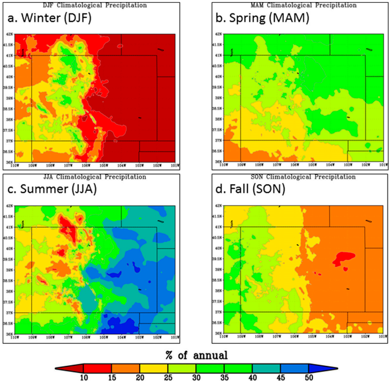
FIG. 6. Seasonal cycle of climatological precipitation based on COOP and SNOTEL data integrated via PRISM [Daly et al. (2002) using 1895–2007 period of record] for (a) winter, (b) spring, (c) summer, and (d) fall. Shading indicates the percentage of the annual precipitation that occurs during the indicated season.
