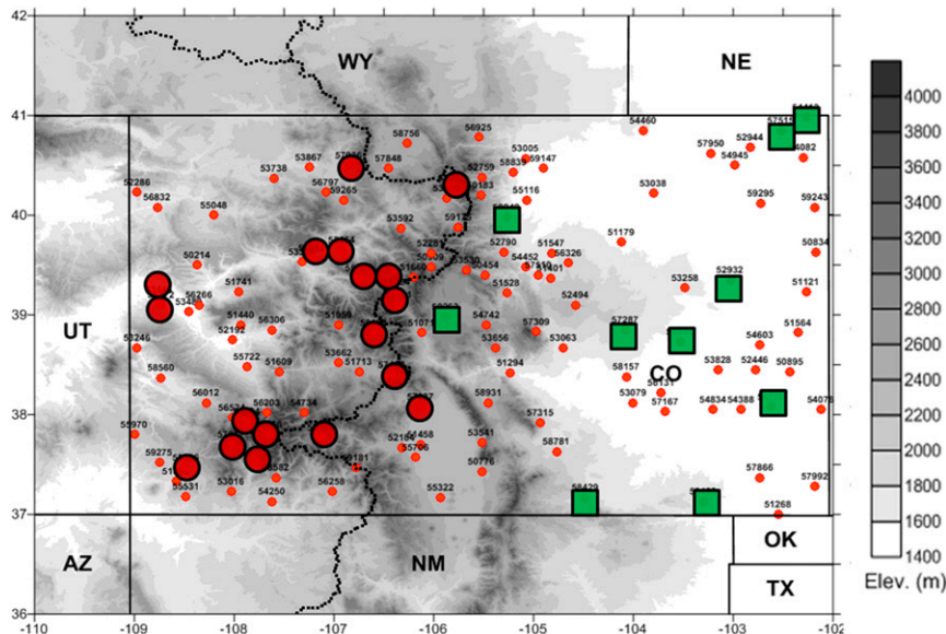
FIG. 7. Comparison of top precipitation events to seasonal climatology. Stations in red circles (green squares) denote those in which <40\% ( >90\% ) of the top 10 daily precipitation events fell during any of the climatologically favored three wettest months and >40\% (none) of the top 10 daily precipitation events occurred during the climatologically driest six months.
