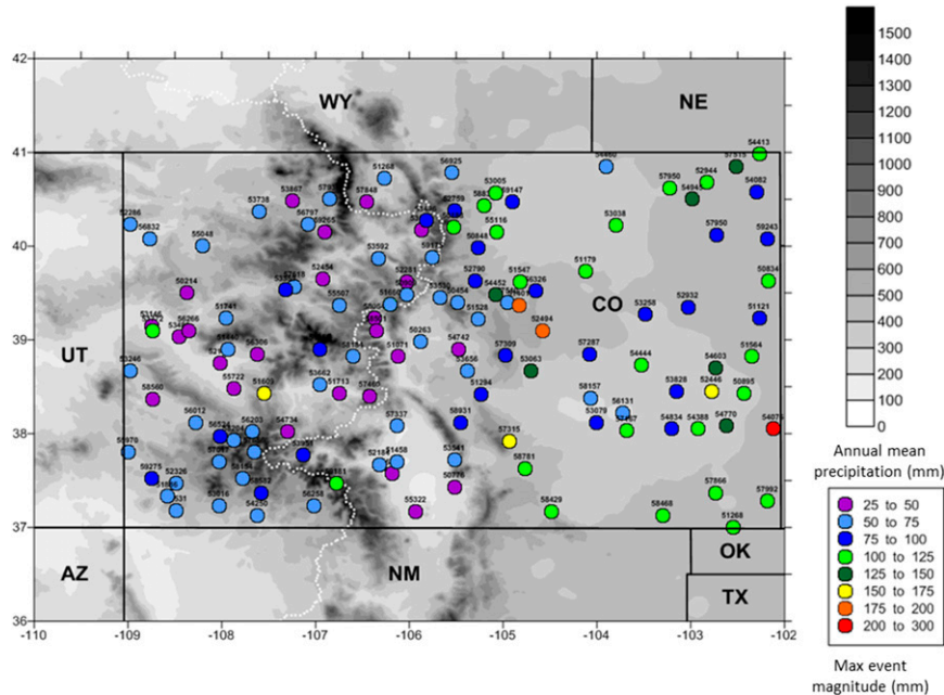
FIG. 1. Max event magnitude (mm) by COOP station for 1951–2010, shaded as in legend at lower right. Annual mean precipitation from PRISM data ( http://prism.oregonstate.edu/ ) based on period of 1981–2010 (mm; gray shading as in legend at upper right). Colorado COOP station ID numbers are listed above circles. Continental Divide is shown by the dashed white line.
