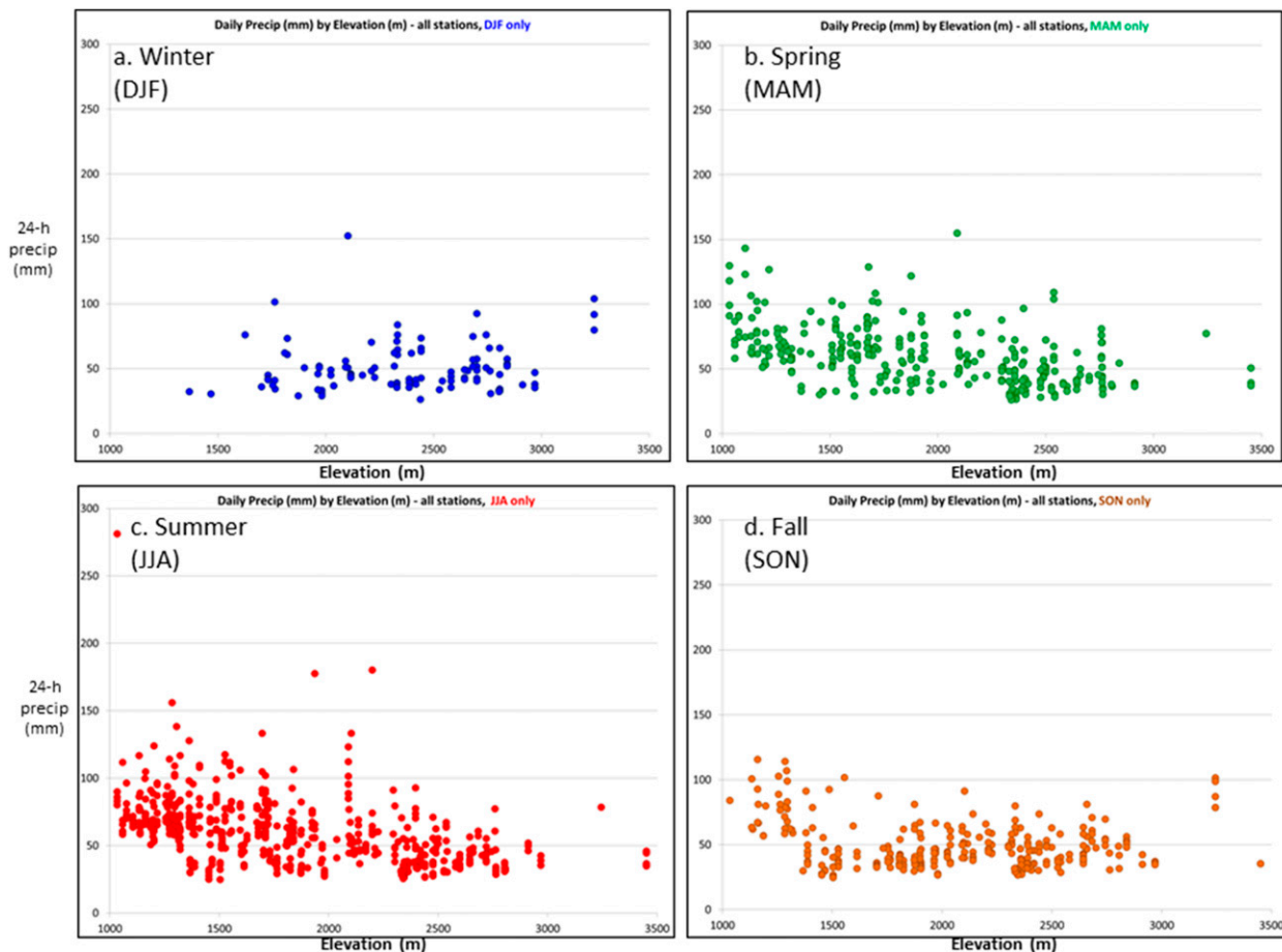
FIG. 4. Seasonal event analysis by station elevation. Each dot represents an individual event by season: (a) winter, (b) spring, (c) summer, and (d) fall. The 24-h precipitation amount is on the y axis (mm) and elevation is on the x axis (m).
