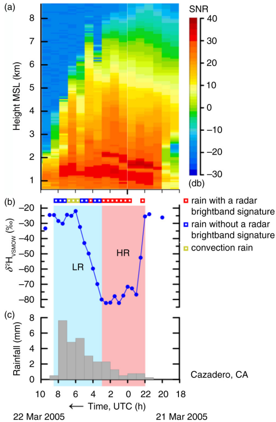
Fig. A5. (a) Time–height section of equivalent radar reflectivity factor with signal-to-noise ratio (SNR), (b) time series of \delta^2 H_{VSMOW} values of 30-min, time-integrated precipitation samples and (c) histogram of hourly rainfall at Cazadero, CA, collected between 18 UTC 21 March 2005 and 10 UTC 22 March 2005. HR, pink panel, higher rainout, decreasing or low \delta^2 H_{VSMOW} values. LR, blue panel, lower rainout, increasing or high \delta^2 H_{VSMOW} values. Open squares indicate objective categorization of the rainfall occurring during selected half-hour periods. Time increases from right to left.
