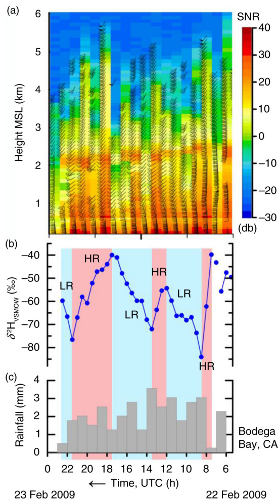
Fig. A30. (a) Time–height series of hourly wind profiles (flags: 25\text{ m s}^{-1} ; barbs: 5\text{ m s}^{-1} ; half-barbs: 2.5\text{ m s}^{-1} ) with signal-to-noise ratio (SNR), (b) time series of \delta^2\text{H}_{\text{VSMOW}} values of 30-min, time-integrated precipitation samples and (c) histogram of hourly rainfall at Bodega Bay, CA, collected between 6 UTC 22 February 2009 and 0 UTC 23 February 2009. HR, pink panels, higher rainout, decreasing or low \delta^2\text{H}_{\text{VSMOW}} values. LR, blue panels, lower rainout, increasing or high \delta^2\text{H}_{\text{VSMOW}} values. Time increases from right to left.
