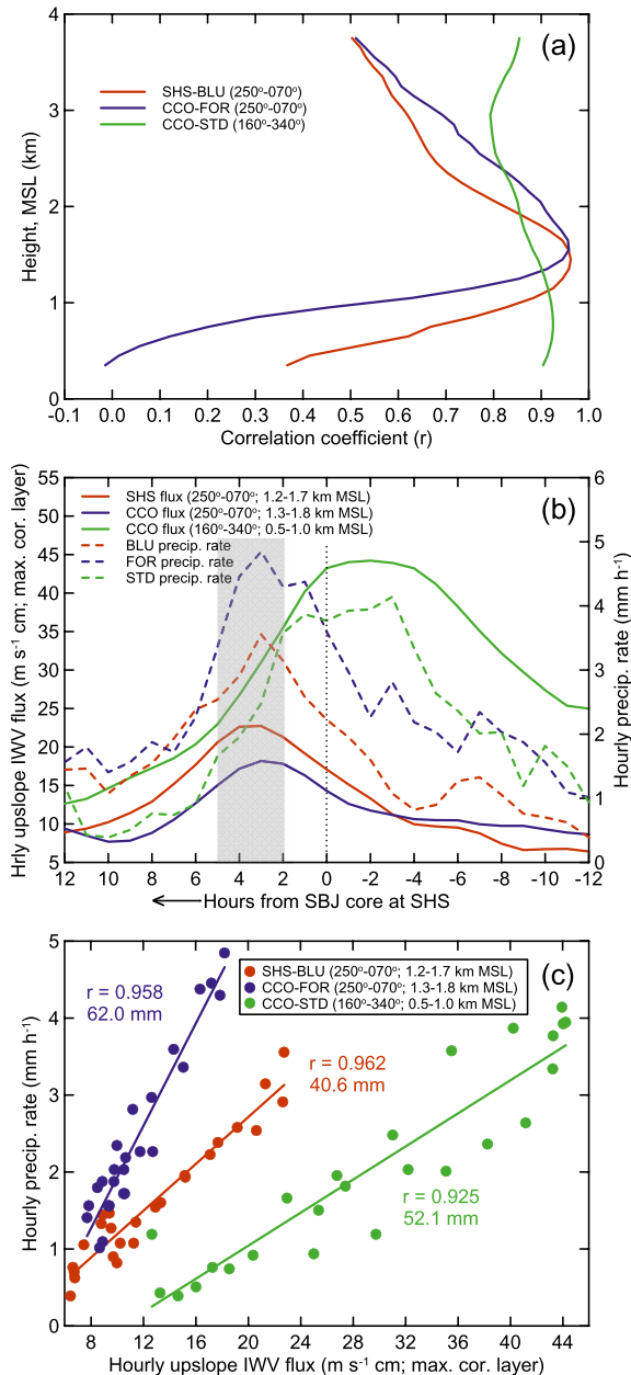
FIG. 8. Composite, 13-case, 24-h duration orographic precipitation analysis from the wind profiler–precipitation gauge couplets at SHS-BLU (red curves; upslope direction from 250°), CCO-FOR (blue curves; upslope direction from 250°), and CCO-STD (green curves; upslope direction from 160°). (a) Vertical profiles of linear correlation coefficient, based on hourly averaged profiles of upslope IWV flux vs hourly precipitation rate. (b) Time series of upslope IWV flux (solid lines) in the layer of maximum correlation coefficient (1.2–1.7 km MSL at SHS-BLU, 1.3–1.8 km MSL at CCO-FOR, 0.5–1.0 km MSL at CCO-STD) and hourly precipitation rate (dashed lines). Time = 0 h (thin vertical dotted line) corresponds to the time of each SBJ core (i.e., V_{\max} ) observed at SHS. The shaded rectangle denotes the 3-h cold-frontal period based on the WRF-RD analysis in Fig. 11. (c) Scatterplot analyses and linear regression fits in the layer of maximum correlation coefficient. Numerical values of correlation coefficient r and composite accumulated precipitation are given.
