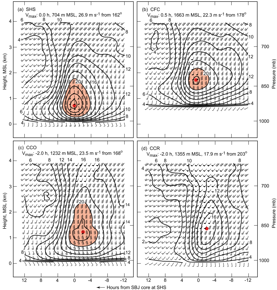
FIG. 5. Composite, 13-case, 24-h duration time-height sections of hourly averaged wind profiles (as in Fig. 2) and Sierra-parallel isotachs ( \text{m s}^{-1} ; directed from 160°; >20 \text{ m s}^{-1} red shaded) at (a) SHS, (b) CFC, (c) CCO, and (d) CCR. Time = 0 h corresponds to the time of each SBJ core (i.e., V_{\text{max}} ) observed at SHS. The red dot in each panel marks the time and altitude of the site-specific V_{\text{max}} , the attributes of which are also given. Time increases from right to left, as in Fig. 2.
