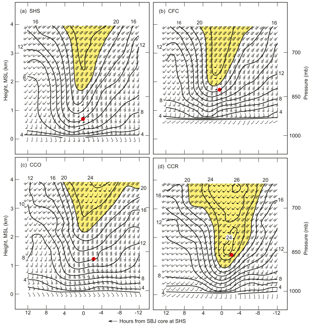
FIG. 6. As in Fig. 5, but for AR-parallel isotachs (directed from 220°; >20 \text{ m s}^{-1} yellow shaded).
