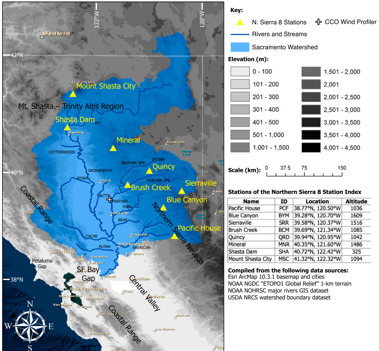
FIG. 1. The locations, IDs, and altitude (m MSL; inset table) of the eight stations that comprise the NS8I (yellow triangles) atop terrain elevation (m; shaded according to scale) and an outline of the Sacramento River watershed (blue shaded) and its tributaries (blue lines). The location of the CCO wind profiler is indicated by the white cross.
