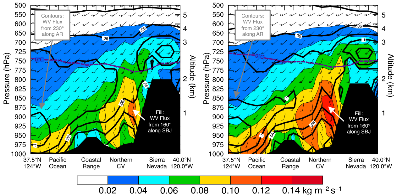
FIG. 4. Composite cross section along an AR-parallel line from 37.5°N, 124°W to 40°N, 120°W (shown in Fig. 3) of the (a) 50 days and (b) top 10 days with EDP that illustrates SBJ water vapor (WV) flux ( \text{kg m}^{-2} \text{s}^{-1} ; shaded according to scale), AR WV flux (contoured every 0.02 \text{ kg m}^{-2} \text{s}^{-1} beginning at 0.02 \text{ kg m}^{-2} \text{s}^{-1} ), and total wind barbs (as in Fig. 2b). The SBJ WV flux is projection of total WV flux along 160^\circ , whereas AR WV flux is projection of total WV flux along 230^\circ .
