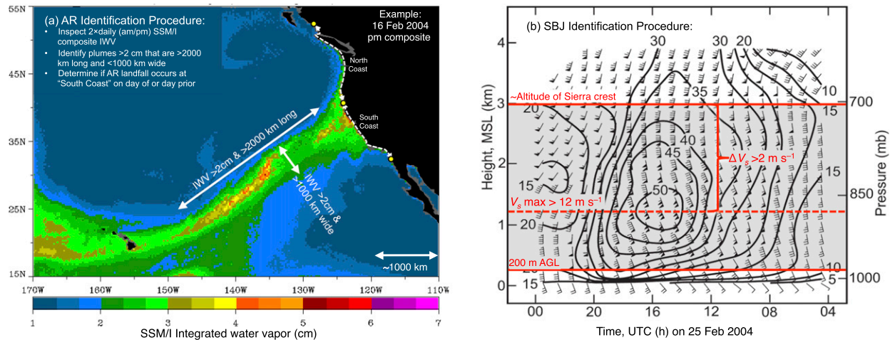
FIG. 2. (a) Annotated SSM/I satellite-based IWV (cm; shaded) on 16 Feb 2004 that illustrates the method used to detect the presence of a landfalling AR in each of the 50 days with EDP. Only ARs making landfall in California are counted [i.e., between 32.5^{\circ} and 41^{\circ} N as in the Neiman et al. (2008b) AR catalog]. (b) Annotated time–height section adapted from Neiman et al. (2010) of hourly averaged wind profiles (flag = 25 \text{ m s}^{-1} ; barb = 5 \text{ m s}^{-1} ; half barb = 2.5 \text{ m s}^{-1} ) and barrier-parallel isotachs ( \text{m s}^{-1} ; directed from 160^{\circ} ) at CCO on 25 Feb 2004 that illustrates the method used to detect the presence of an SBJ.
