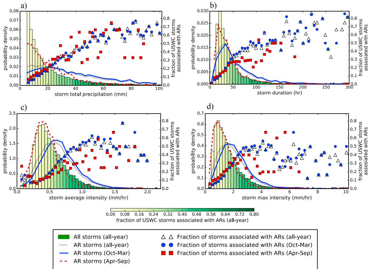
Figure 4. PDF of (a) storm totals, (b) storm duration, (c) average storm intensity, and (d) maximum storm intensity for all storms, all-year AR-associated storms, cool season (October–March) AR-associated storms, and warm season AR-associated storms in USWC coastal grid cells are shown by bars, dotted black lines, solid blue lines, and dashed red lines, respectively. The colors of bars represent the fraction of storms in each bin that are associated with ARs. The fraction of all-year, cool season, and warm season storms that are associated with ARs is shown by white triangles, blue circles, and red squares, respectively.
