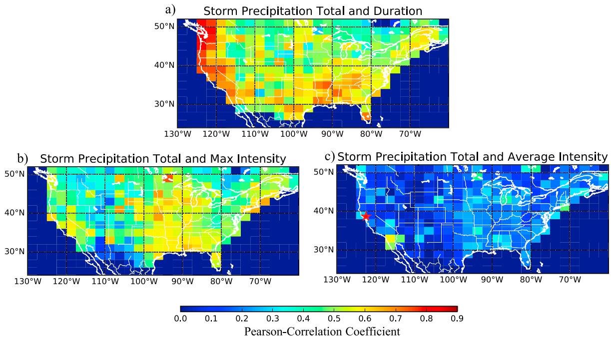
Figure 2. Spatial map of Pearson correlation coefficients of storm precipitation total with (a) storm duration, (b) storm maximum intensity, and (c) storm average intensity for storms observed from 1948 to 2002.
