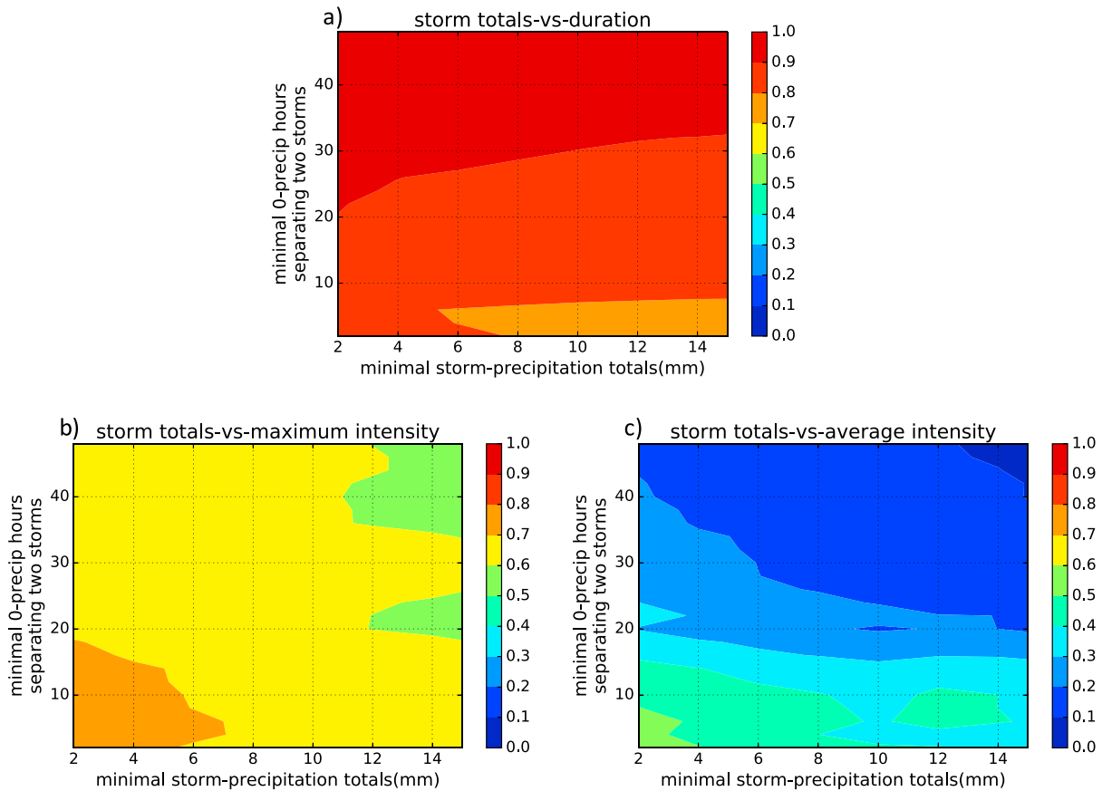
Figure 3. Pearson correlation coefficient of precipitation totals with duration, maximum intensity, and average intensity at Cazadero station (shown by red star in Figure 2c), using 2 min observations from 2011 to 2016.
