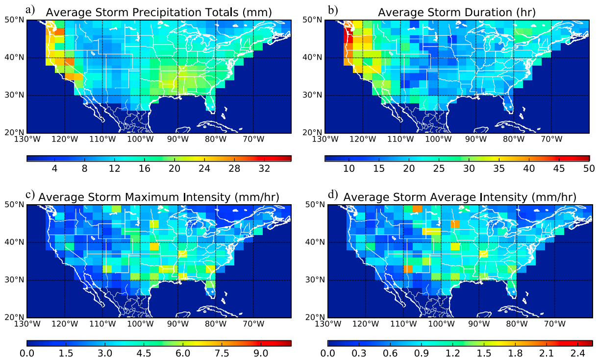
Figure 1. Climatology of (a) storm total precipitation, (b) storm duration, (c) storm maximum intensity, and (d) storm average intensity based on gridded hourly precipitation observations from 1948 to 2002.
