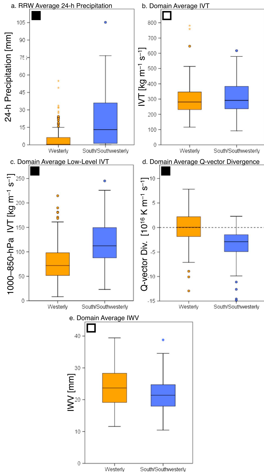
Figure 4. Box and whisker plots of Russian River Watershed (a) area average 24 h precipitation (mm), (b) domain average IVT ( \text{kg m}^{-1} \text{s}^{-1} ), (c) domain average lower tropospheric (1000–850 hPa) IVT ( \text{kg m}^{-1} \text{s}^{-1} ), (d) domain average Q-vector divergence ( 10^{16} \text{K m}^{-1} \text{s}^{-1} ), and (e) domain average IWV (mm) for westerly (orange) and south-southwesterly (blue) ARs. The boxes represent the interquartile range of the data, and the whiskers represent upper and lower quartiles of the data. The horizontal line within the boxes is the median value. The colored dots represent outliers, and the asterisks represent extreme outliers. The box in the top left corner of each panel indicates the result of the independent samples t test with 95% confidence (white indicates significantly statistically similar means and black indicates significantly statistically different).
