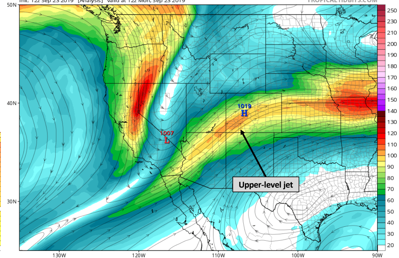
GFS 250mb Wind Speed/Streamlines (kt) & MSLP Extrema (mb) Init: 12z Sep 23 2019 [Analysis] valid at 12z Mon, Sep 23 2019
