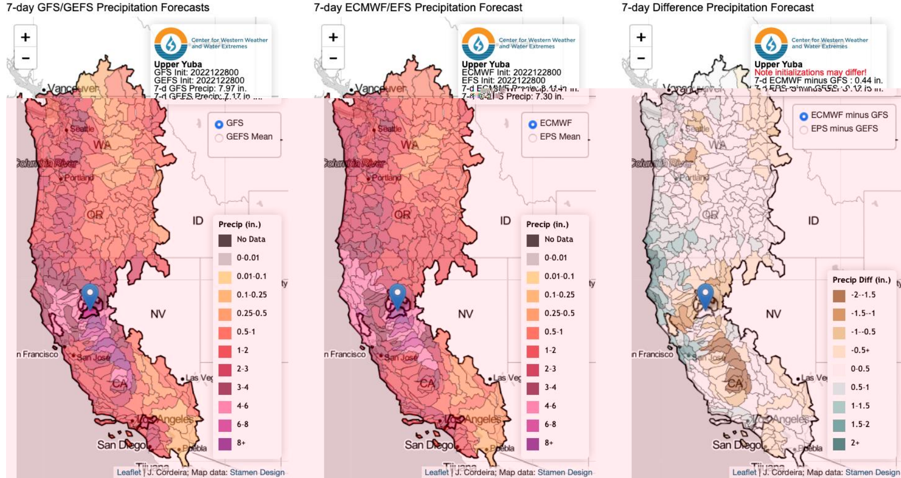
GFS/GEFS and ECMWF/EFS 7-day Watershed Precipitation Forecast (initialized 0000 UTC 28 December 2022)
