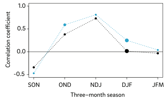
b) Seasonal skill at 1 month lead time
