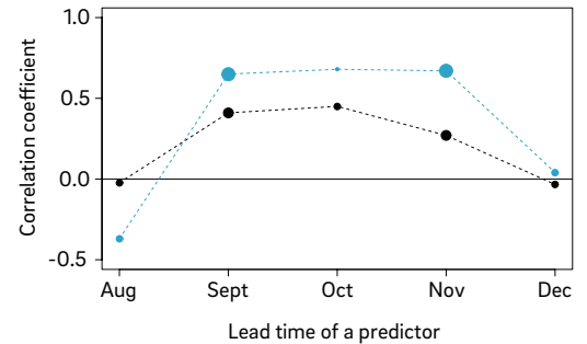
a) JFM 2020 skill at various lead times
