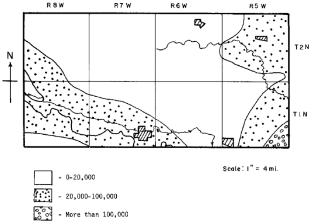
Figure 14: Generalized transmissivity map of study area (Redrawn from LRNRD, 1985, and LBNRD, 1986)
