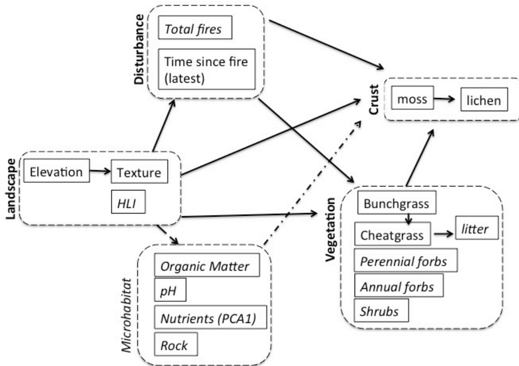
Figure 9: Conceptual diagram of hypothesized relationships between unobserved factors (dotted boxes) and observed variables (rectangles). Arrows indicate directed relationships. Observed variables in italics and dotted paths are considered nonessential and are assessed for importance only in relation to the rest of the model. Potential feedback relationships are not modeled.
