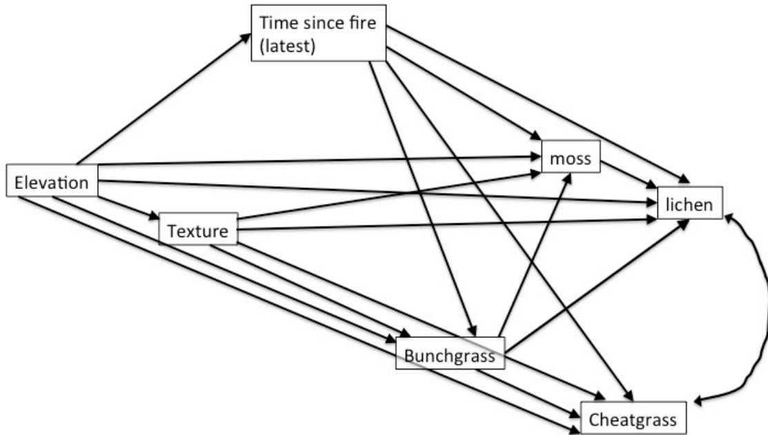
Figure 11: Proposed pathways from landscape, disturbance, and vegetation pathways to biological soil crust cover. Variables are defined in Table 7. Double-headed curved arrow indicates unresolved correlation between the errors of B. tectorum and lichen cover. Single headed arrows indicate directed relationships between variables. Error terms for endogenous variables are not shown.
