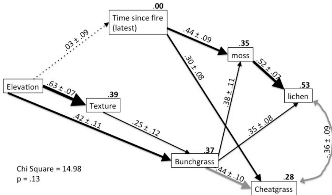
Figure 12: Final model with fit, Chi-square = 14.98, p = 0.13 , df = 10 . Arrows are drawn proportional to standardized regression weight and values are displayed with bootstrap estimates of standard error. Positive correlations are in black and negative correlations in grey. Error terms for endogenous variables are not shown. Dotted line is nonsignificant. R^2 values are displayed in bold above each variable.
