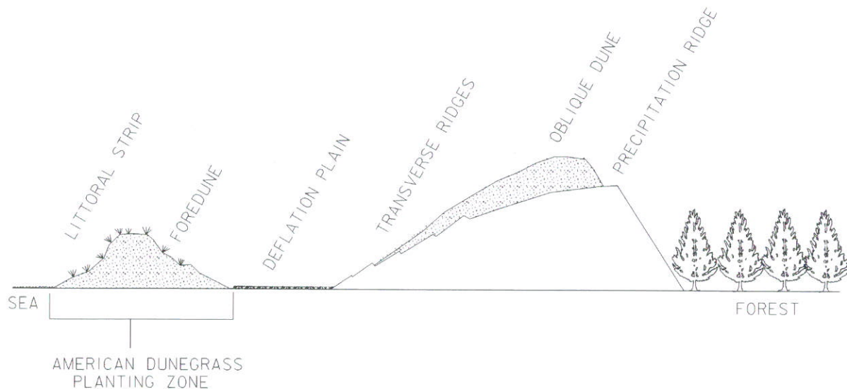
Figure 2-1 Dune Land Features Profile
