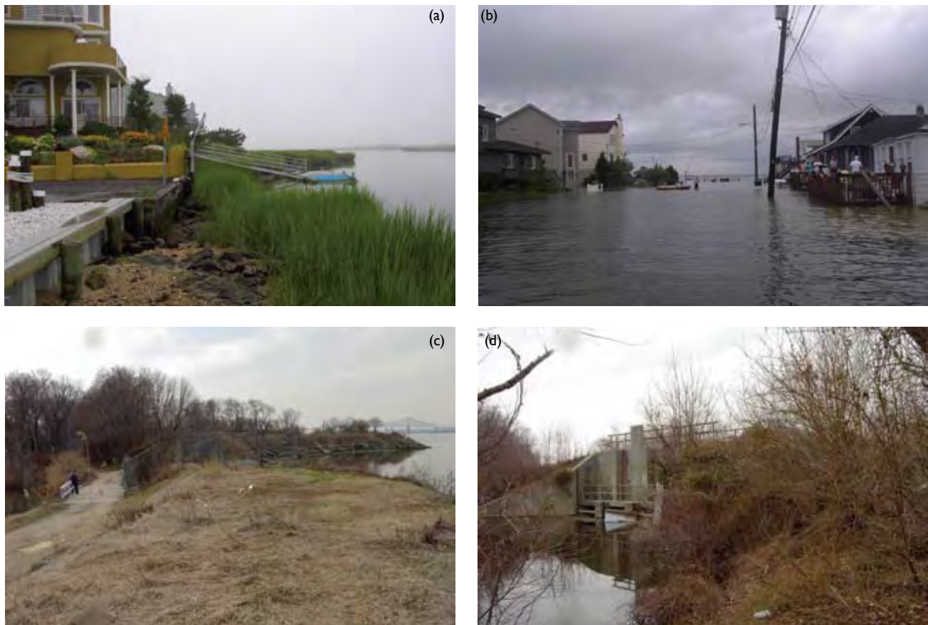
Figure 11.4 Vulnerability of New Jersey's coastal zone. (a) Wetland fringe lacks room for wetland migration (Monmouth, August 2003). (b) Low bay sides of barrier islands are vulnerable to even a modest storm surge (Ship Bottom, September 2, 2006). (c) Gibbstown Levee and (d) associated tide gate protect lowlying areas of Greenwich Township (March 2003) [Photo source: ©James G. Titus, used with permission].
