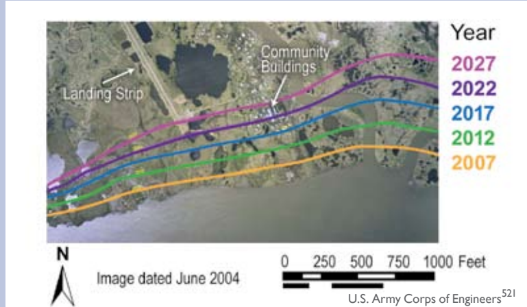
Many of Alaska’s coastlines are eroding rapidly; the disappearance of coastal land is forcing communities to relocate. The 2007 line on the image indicates where Newtok, Alaska’s shoreline had eroded to by 2007. The other lines are projected assuming a conservative erosion rate of 36 to 83 feet per year; however, Newtok residents reported a July 2003 erosion rate of 110 feet per year.
