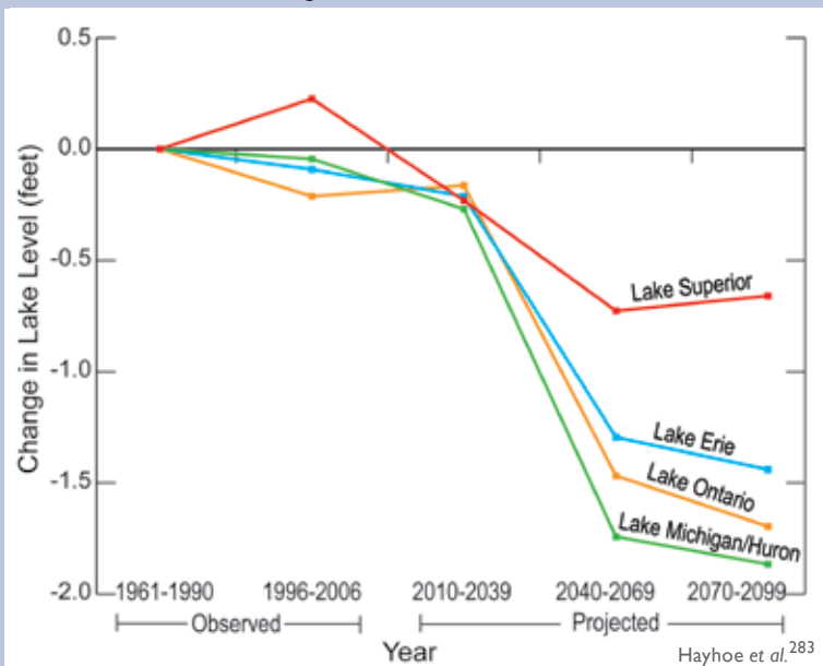
Average Great Lakes levels depend on the balance between precipitation (and corresponding runoff) in the Great Lakes Basin on one hand, and evaporation and outflow on the other. As a result, lower emissions scenarios 91 with less warming show less reduction in lake levels than higher emissions scenarios. 91 Projected changes in lake levels are based on simulations by the NOAA Great Lakes model for projected climate changes under a higher emissions scenario. 91
