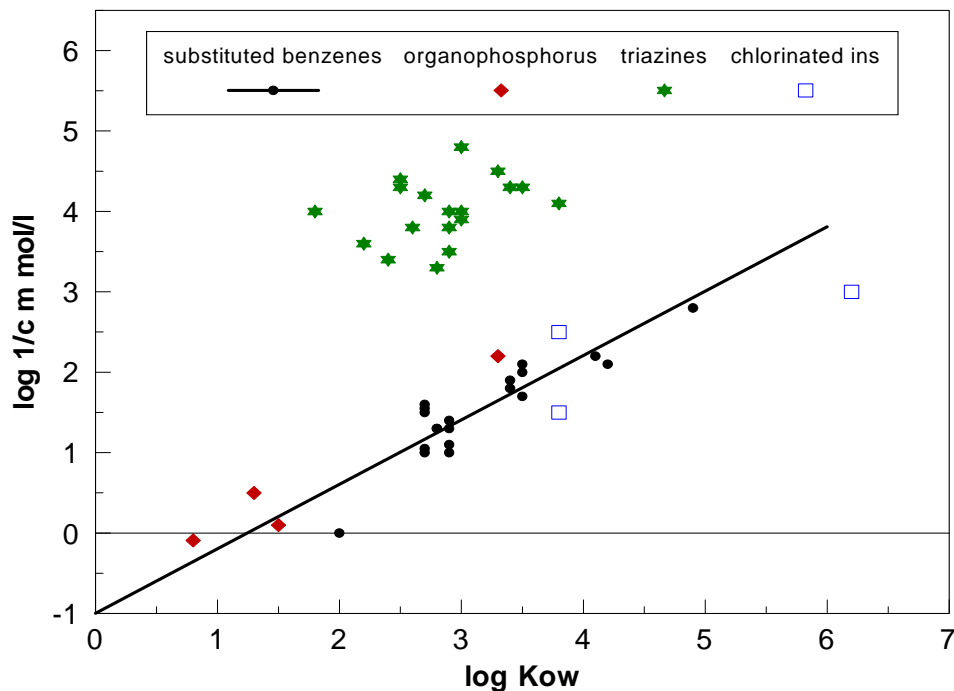
Figure 2 – Relationship between toxicity on algae (Log 1/EC50) and Log Kow for chemicals with a specific (triazines) and a non-specific (all others) toxicological mode of action on algae (Vighi 2006).
