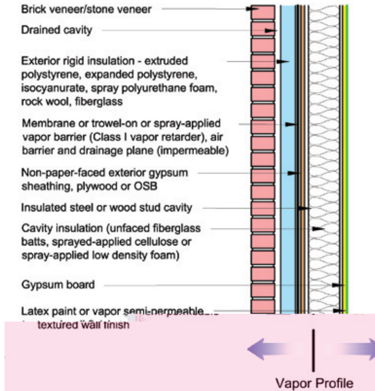
Figure 2-11 Frame Wall with Exterior Rigid Insulation with Cavity Insulation and Brick or Stone Veneer
