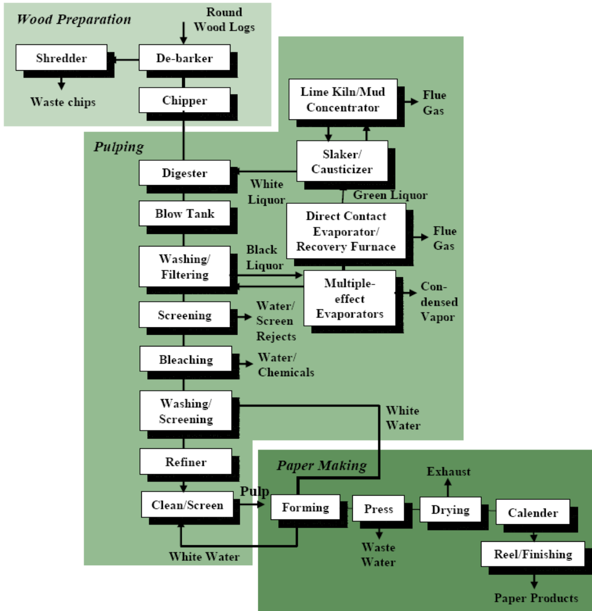
Figure 1. Flow Diagram of the Pulp and Paper Manufacturing Process (Staudt 2010)
