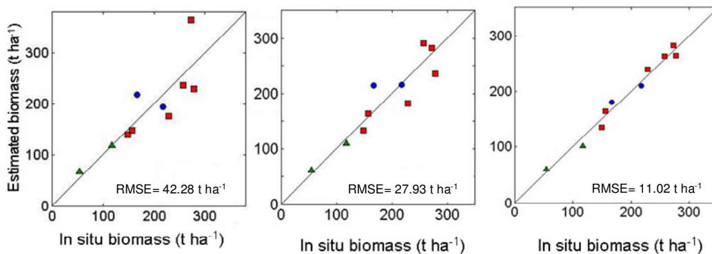
Figure 9: Comparison of estimated and in situ biomass for a) inversion of HV intensity data, b) inversion using HV & HH intensity data together with Pol-InSAR height, and c) inversion using HV & HH intensity data, Pol-InSAR height and the HV Ground to Volume backscatter ratio. Squares: spruce stands, circles: pine stands, and triangles: birch stands.
