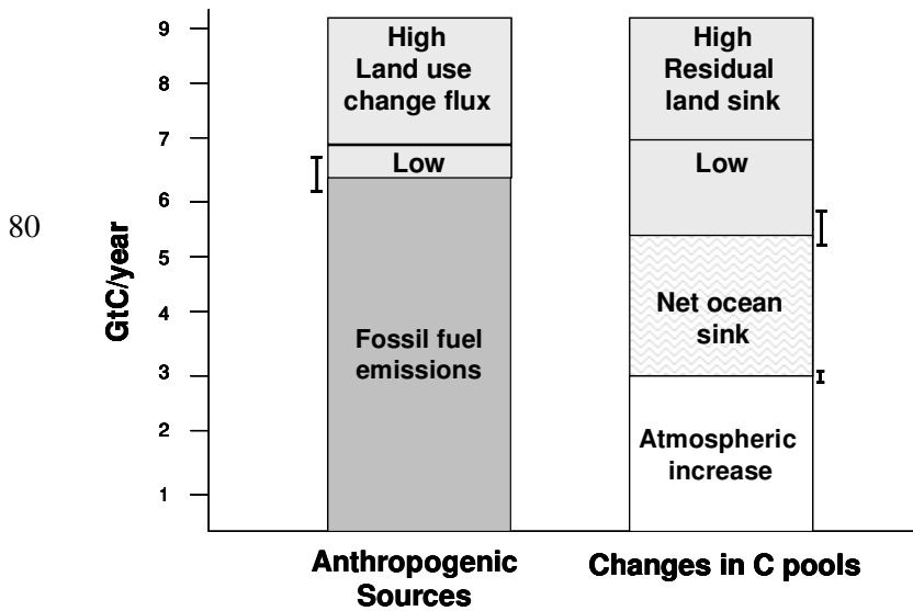
85 Figure 1. Bar chart showing the anthropogenic carbon sources and the associated annual net fluxes to the carbon pools for the 1990s, with units given as GtC\ yr^{-1} . The uncertainties in the well-constrained terms (fossil fuel emissions, the atmospheric increase in CO_2 and the net ocean sink) are indicated by the error bars. The land use change flux is poorly constrained and the chart indicates the range of estimates, from 90 low to high, of this quantity. In order to achieve carbon balance, there must be take-up of CO_2 by the land surface, and the corresponding low and high estimates of this “residual land sink” are indicated. The data for this figure are taken from IPCC (2007).
