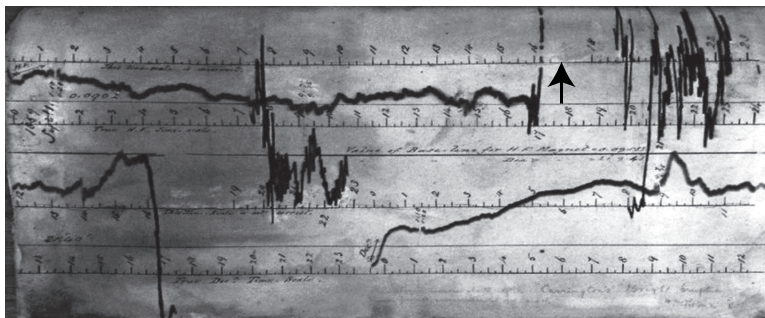
Figure 8: Horizontal magnetic field strength (upper) and direction (lower) for the full day of 1 September 1859 at Kew Observatory, during the Carrington Event. The arrow represents a magnitude of \approx 100 nT. Just left of the arrow, the field strength appeared to go far off scale.
