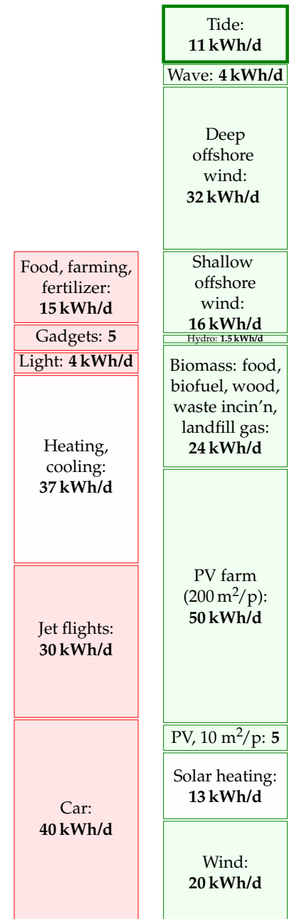
Figure 14.10. Tide.
