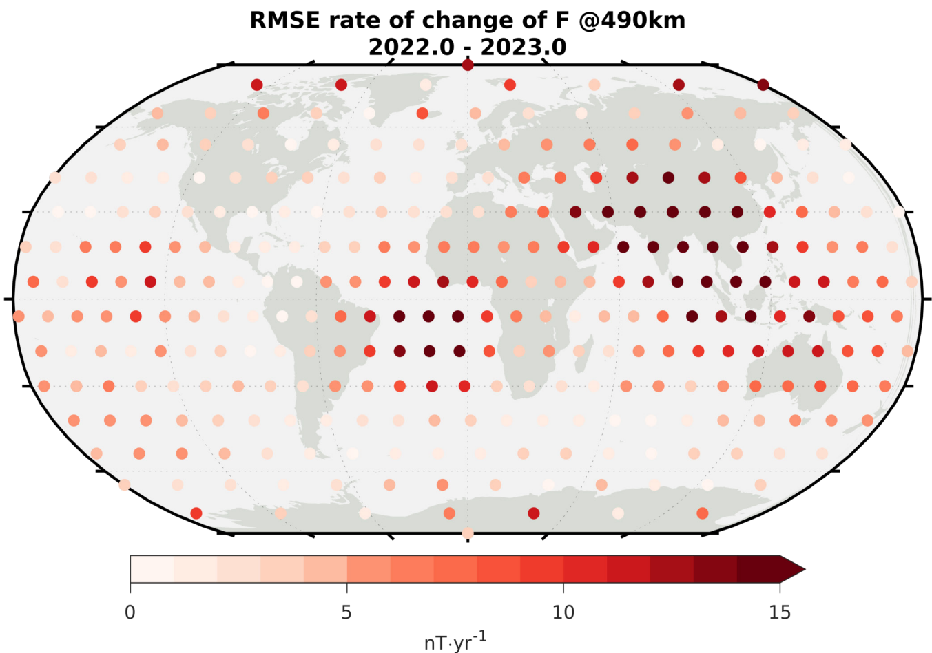
Figure 2: RMSE between prediction of WMM2020 SV of total intensity ( F ) and geomagnetic virtual observatory data in 2022.
