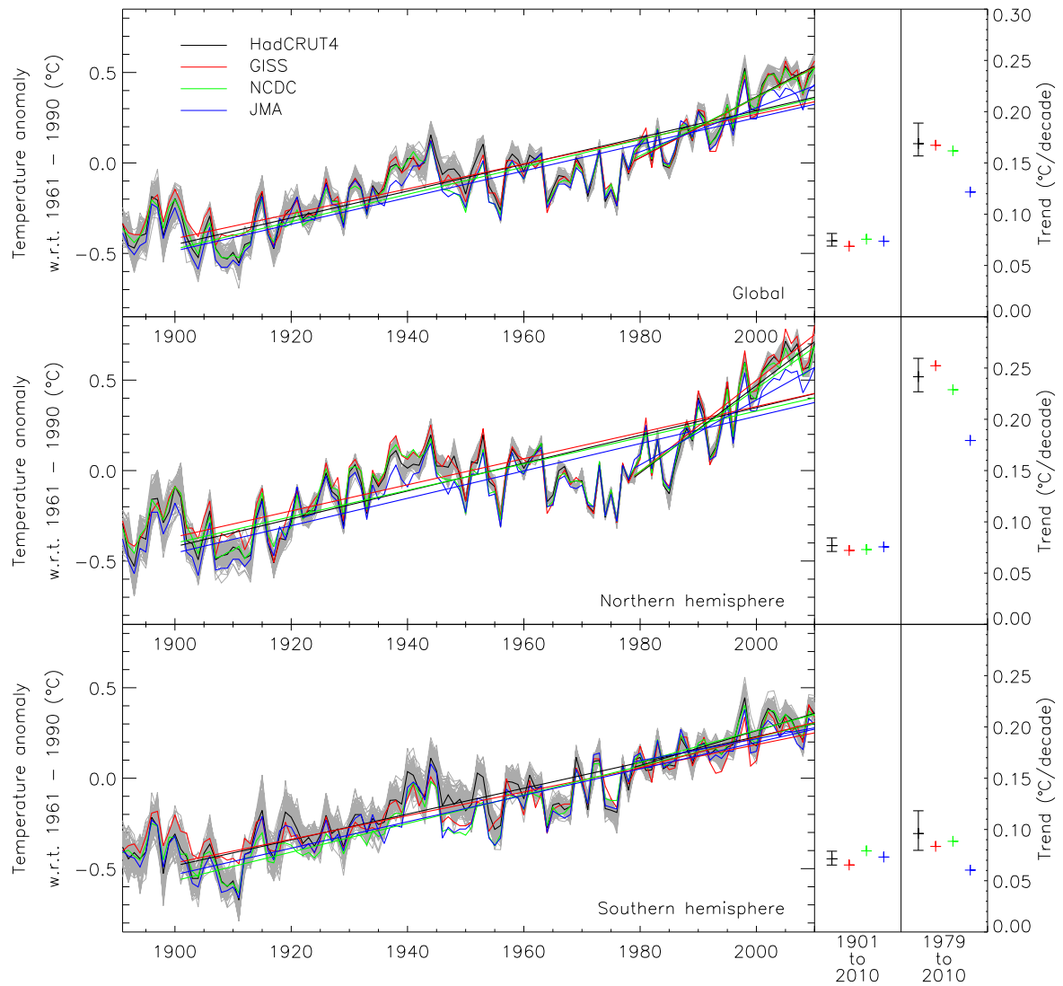
Figure 11 – Annual temperature anomaly development in the HadCRUT4, GISS, NCDC and JMA surface temperature analyses. Least squares linear trends are shown on the right for the periods of 1901 to 2010 and of 1979 to 2010. Individual ensemble member realizations of HadCRUT4 are shown in grey. Uncertainty ranges in linear trends for HadCRUT4 data are computed as the 2.5% and 97.5% ranges in linear trends observed in the HadCRUT4 ensemble.
