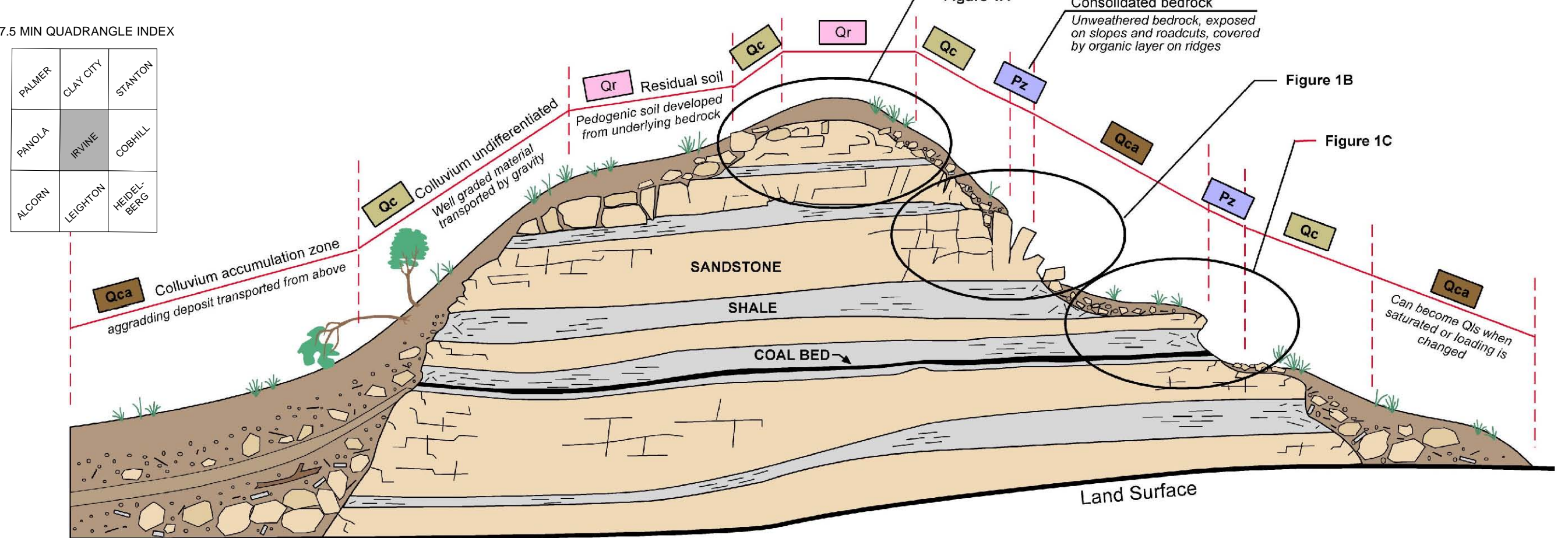
Figure 1. Conceptual model of the geomorphic processes in the Irvine 7.5-minute quadrangle
