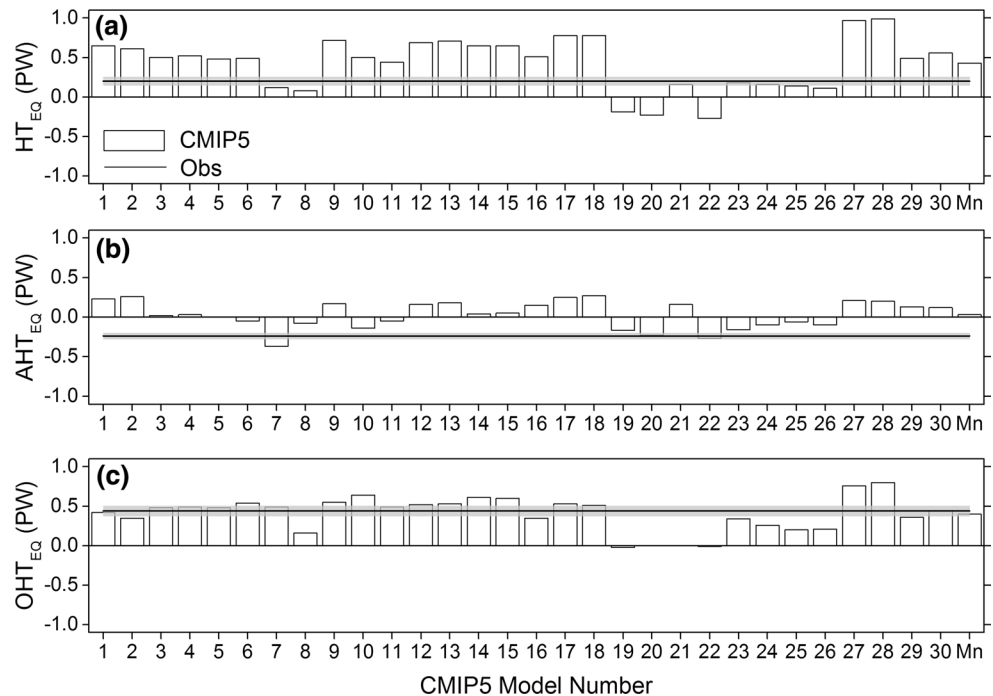
Fig. 4 Cross-equatorial heat transport for a total ( HT_{EQ} ), b atmosphere ( AHT_{EQ} ) and c ocean ( OHT_{EQ} ) from the first 30 CMIP5 models in Table 1 and from observations ( thick line ). “Mn” corresponds to the multi-model mean value. Gray shading represent the observational uncertainty
