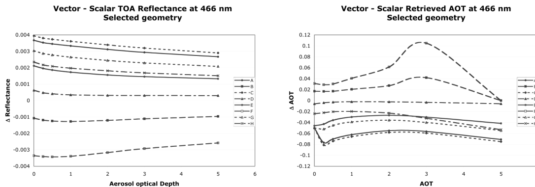
Figure 13: Difference between vector- and scalar- derived reflectance (a) and retrieved AOD (b) at 0.466 \mu\text{m} , for eight example sun/surface/satellite geometries as a function of the input AOD.
