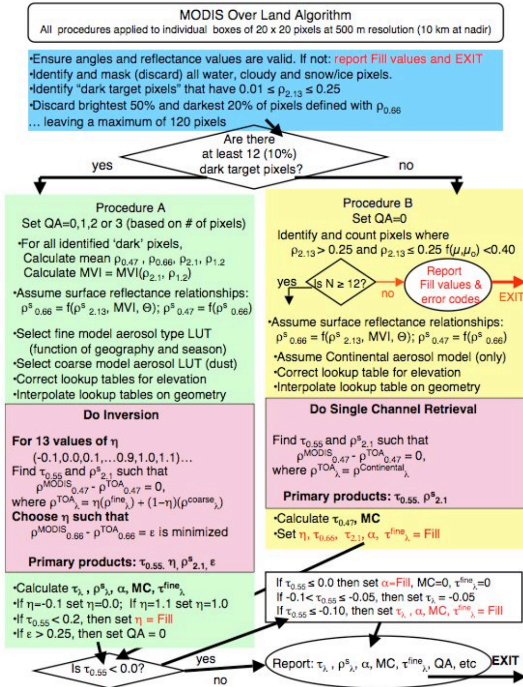
Figure 20: Flowchart illustrating the derivation of aerosol over land for V5.2.
