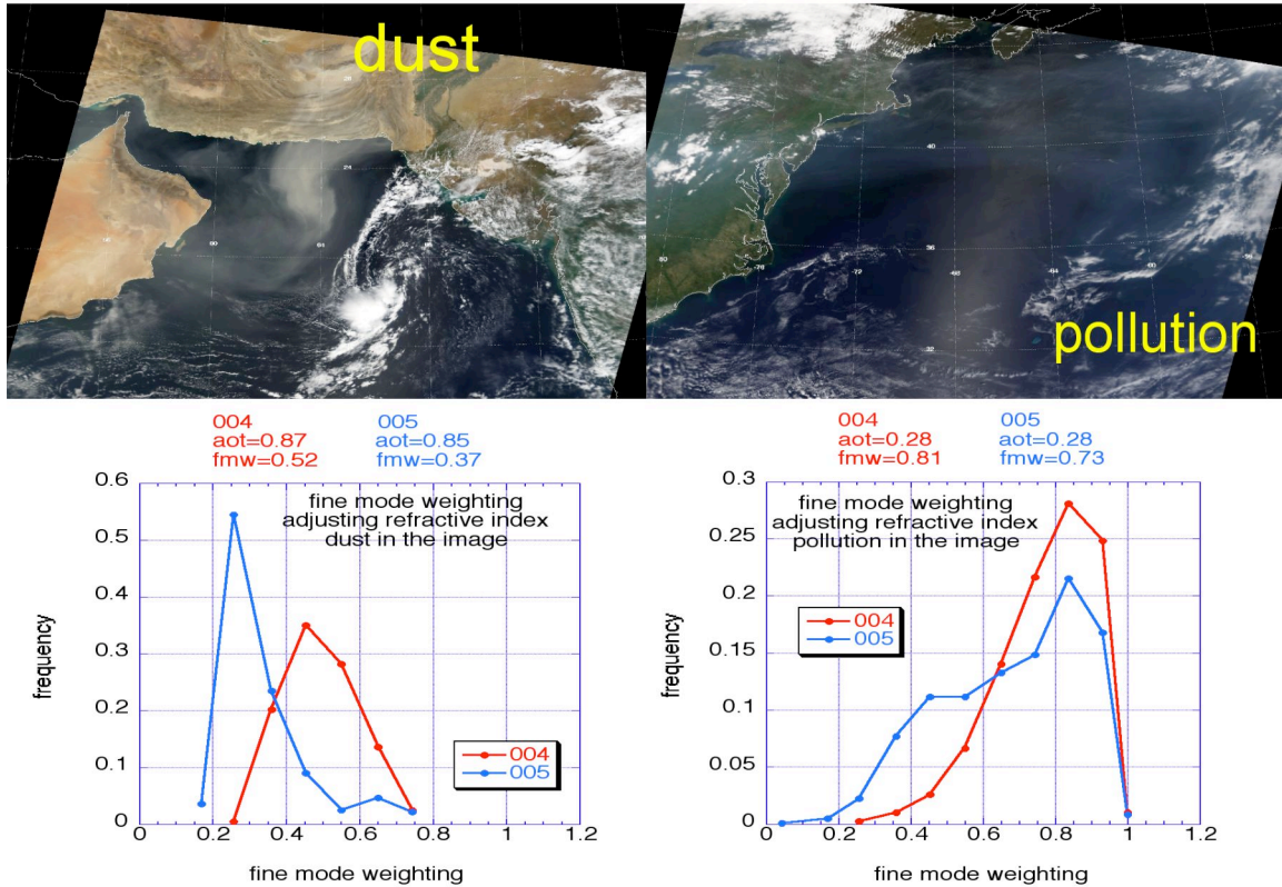
Figure 3: In dusty situations the Collection 004 (red) data reported a too high proportion of fine mode aerosols with average Fine Weighting (FW or FMW) of \sim 0.5 . In smoke or pollution aerosols it retrieved roughly the correct fmw of \sim 0.8 . Using the new refractive indices in the three coarse modes, the Collection 005 (blue) retrievals report less fine mode particles in the dust (FW reduces to \sim 0.3 ), but there is still a high frequency of predominately fine mode particles retrieved in the pollution episode. Note that the mean AOD (AOT) remains the same in the two collections.
