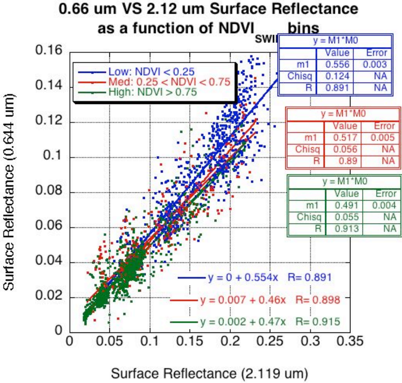
Figure 19: 0.66 \mu\text{m} versus 2.12 \mu\text{m} surface reflectance as a function of bins of NDVI_{SWIR} values (low, medium and high). Both standard regression and “forced through zero” are plotted.
