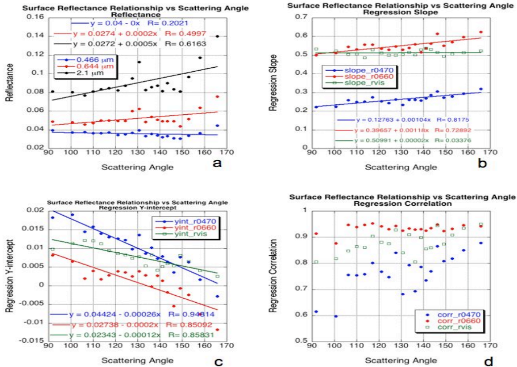
Figure 16: VIS/SWIR surface reflectance relationships as a function of scattering angle. The data were sorted according to scattering angle and put into 20 groups of equal size (about 230 points for each scattering angle bin). On all subplots, each point is plotted for the median value of scattering angle in the bin. Part (a) plots median values of reflectance at each channel as a function of the scattering angle. Linear regression was calculated for the 230 points in each group. The slope of the regression (for each angle bin) is plotted in (b), the y-intercept is plotted in (c) and the regression correlation is plotted in (d). Note for (b), (c) and (d) that 0.47 \mu\text{m} vs 2.12 \mu\text{m} (r0470) is plotted in blue, 0.66 \mu\text{m} vs 2.12 \mu\text{m} (r0660) is plotted in red and 0.47 vs 0.66 \mu\text{m} (rvis) is plotted in green.
