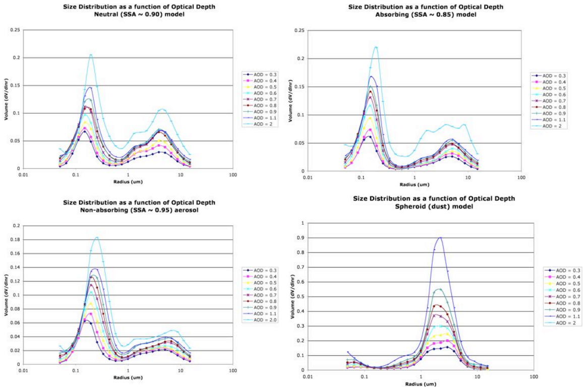
Figure 11: Aerosol size distribution as a function of optical depth for the three spherical (neutral, absorbing and non-absorbing) and spheroid (dust) models identified by clustering of AERONET.
