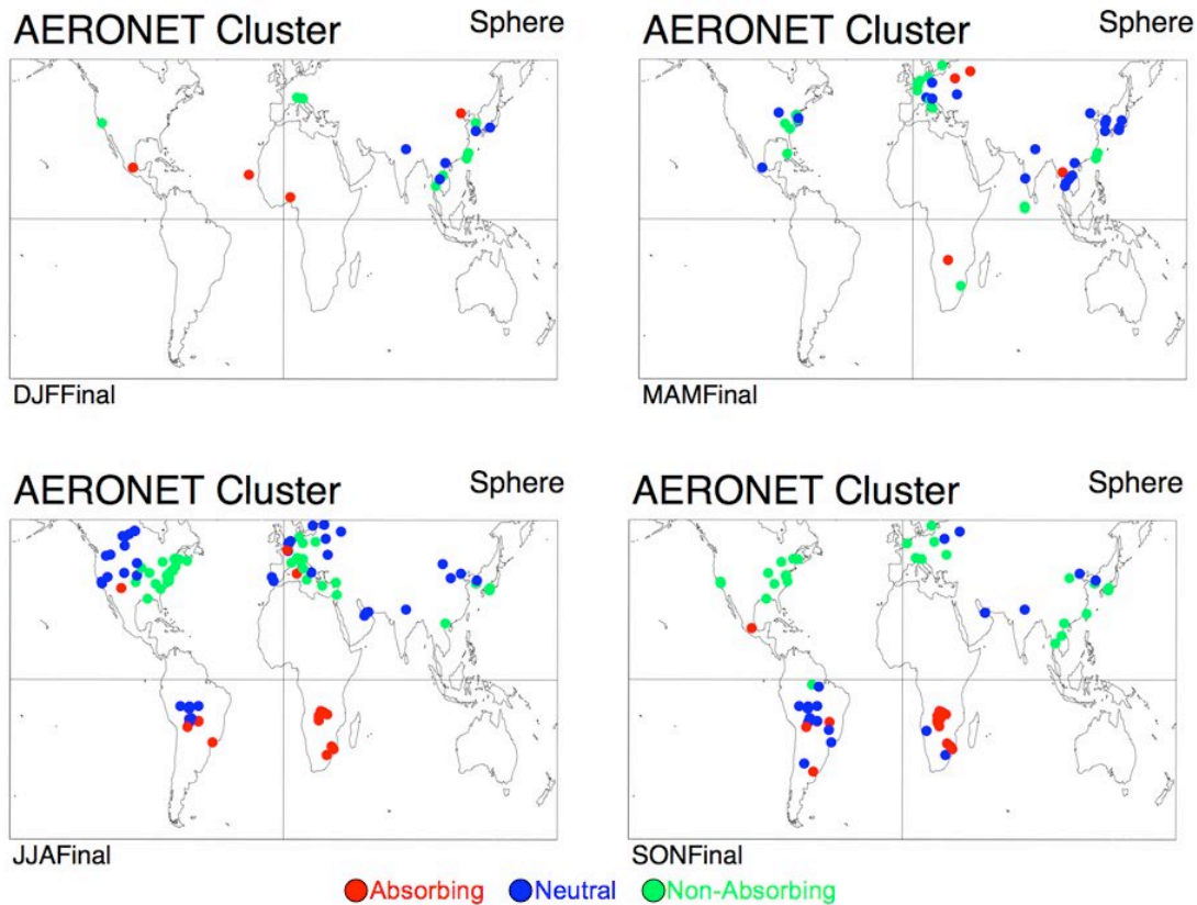
Figure 9: Final spherical aerosol model type designated at each AERONET site per season. Colors represent absorbing (SSA ~ 0.85), neutral (SSA ~ 0.90) and non-absorbing (SSA ~ 0.95), respectively.
