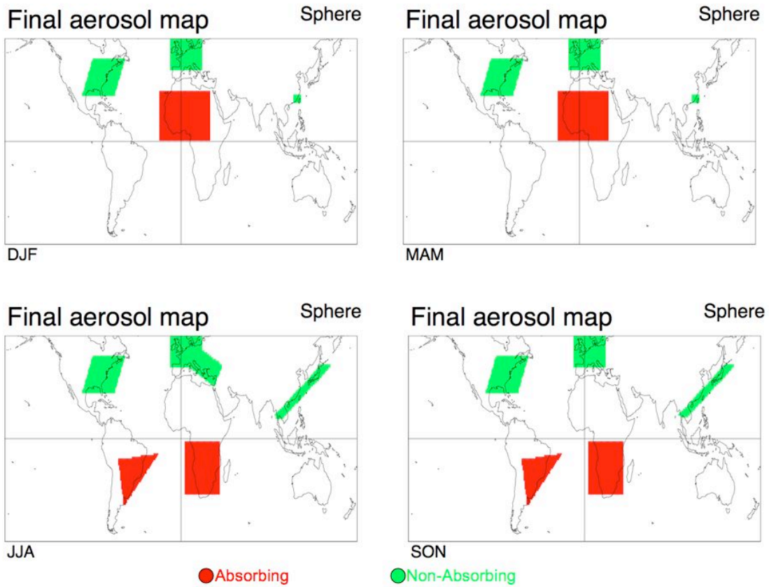
Figure 10: Final spherical aerosol model type designated at 1^\circ \times 1^\circ gridbox per season. Red and green represent absorbing (SSA \sim 0.85 ) or non-absorbing (SSA \sim 0.95 ) models, respectively. Neutral (SSA \sim 0.90 ) is assumed everywhere else.
