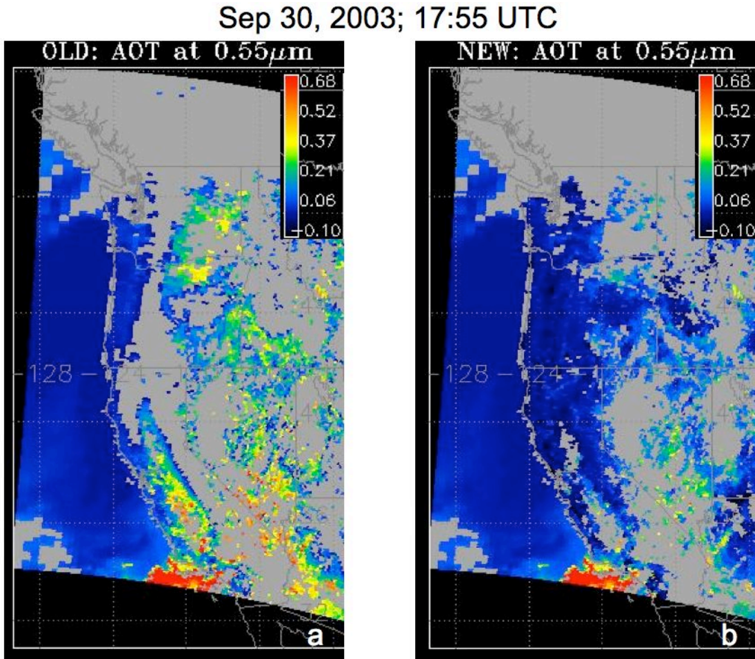
Figure 26: Retrieved AOD at 0.55 \mu\text{m} for Old V5.1 (a) and New V5.2 (b) over California for 30 September 2003. The color scale is the same for both plots. Note the increase in the retrieval spatial coverage and reduction in surface contamination for V5.2.
