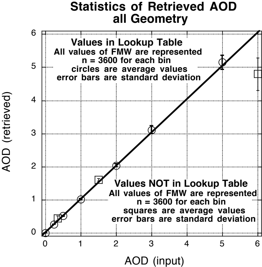
Figure 21: Scatter diagram of the retrieved AOD versus the input AOD. The open shapes correspond to the average of the solutions for each inputted AOD, where there are 3600 combinations of geometry and input FMW. The error bars are the standard deviation of the 3600 inputs. The open circles represent cases where the inputted AOD are included in the V5.2 lookup table, whereas the open squares represent inputted AOD that are not in the LUT.
