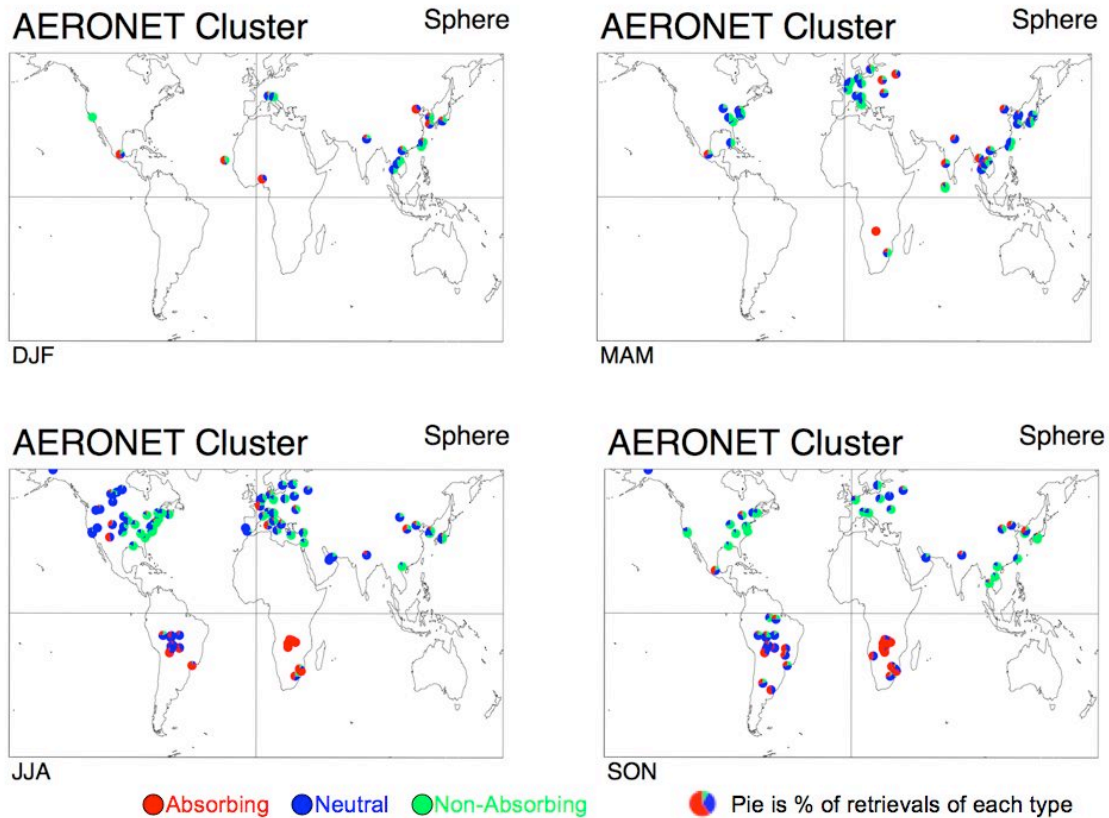
Figure 8: Percentage (pie charts) of spherical aerosol model type retrieved at each AERONET site per season. Colors represent absorbing (SSA ~ 0.85), neutral (SSA ~ 0.90) and non-absorbing (SSA ~ 0.95), respectively.
