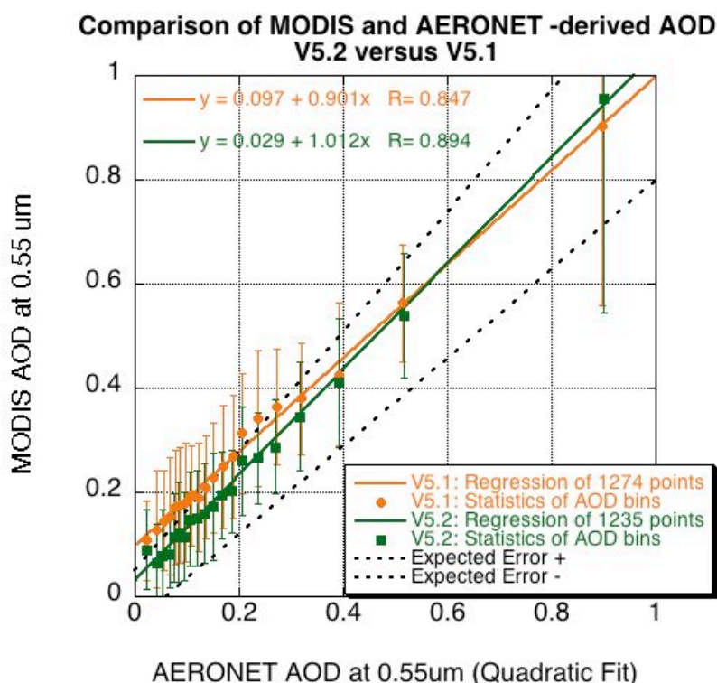
Figure 30: MODIS AOD over land retrieved at 0.55 \mu\text{m} , compared with AERONET AOD interpolated to 0.55 \mu\text{m} . The solid shapes and error bars represent the mean and standard deviation of the MODIS retrievals, in 20 bins of AERONET-derived AOD. Both the retrievals from V5.1 (orange) and V5.2 (green) are shown. The regressions (solid lines) are for the cloud of all points (not shown). The expected errors for MODIS ( \pm 0.05 \pm 0.15\tau ) are also shown (dashed lines).
