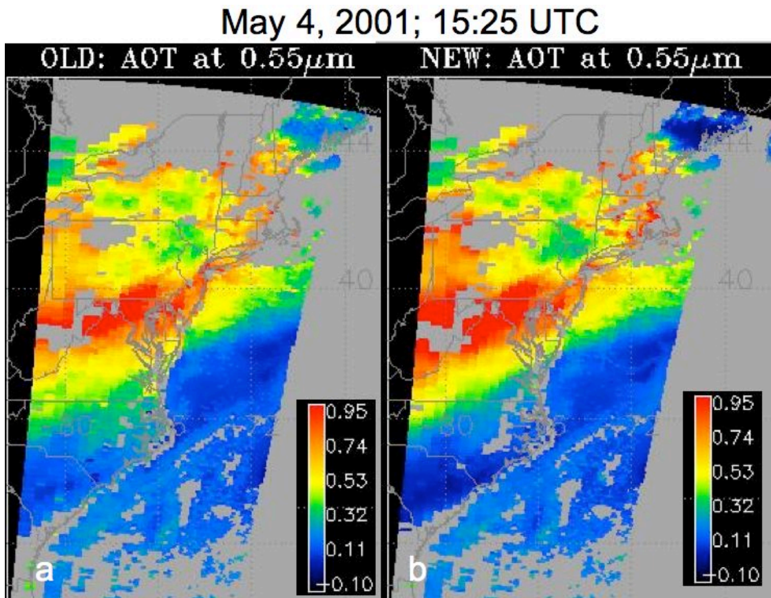
Figure 27: Retrieved AOD at 0.55 \mu\text{m} for Old V5.1 (a) and New V5.2 (b) over the Mid-Atlantic U.S. for 4 May 2001. The color scale is the same for both plots. Note the slight improvement of land/ocean continuity in V5.2.
