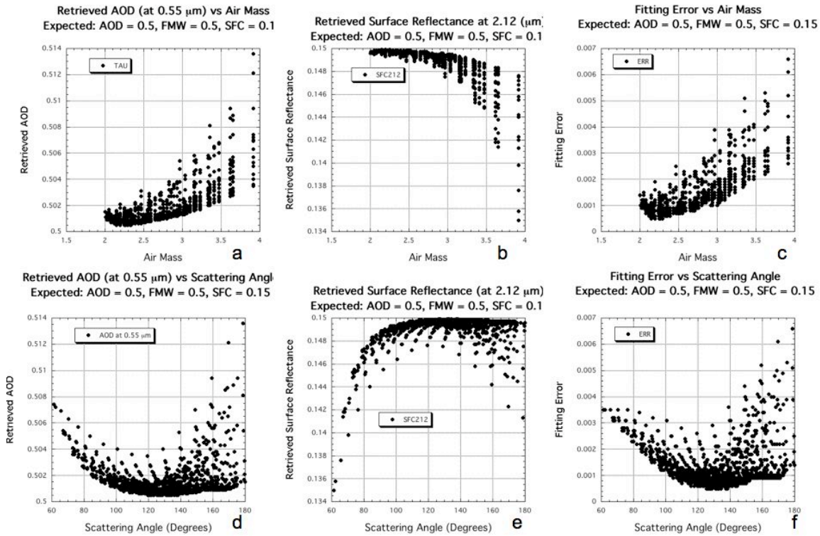
Figure 23: Retrieved MODIS products as a function of Air Mass (a-c) and Scattering Angle (d-f) for given atmospheric conditions ( \tau=0.5 , \eta=0.5 and \rho_{2.12}^s=0.15 ) and 720 LUT geometrical combinations. The retrieved AOD is plotted in (a) and (d), the 2.12 surface reflectance in (b) and (e) and the fitting error is plotted in (c) and (f). Note that in all cases, the FMW value of 0.5 was retrieved exactly.
