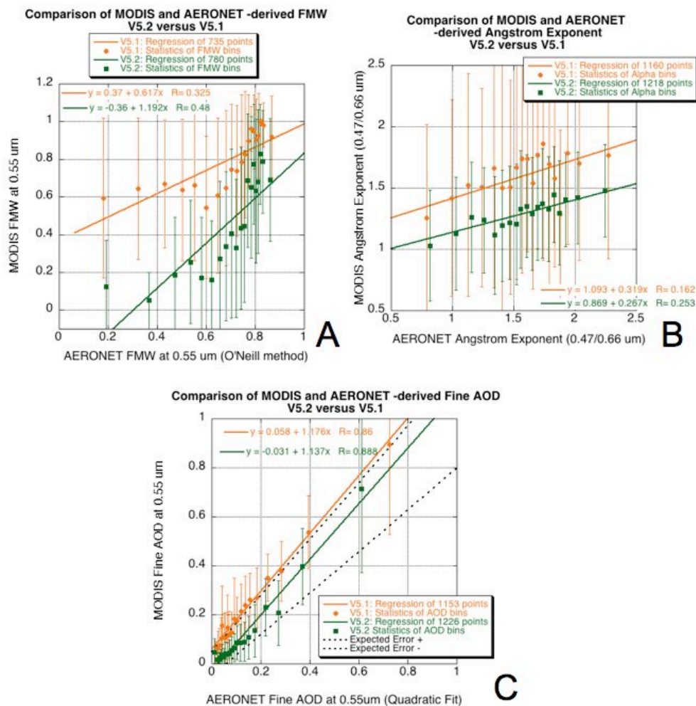
Figure 31: MODIS aerosol size retrievals compared with AERONET derived products. The solid shapes and error bars represent the mean and standard deviation of the MODIS retrievals, in 20 bins of AERONET-derived product. Both the retrievals from V5.1 (orange) and V5.2 (green) are shown. The regressions (solid lines) are for the cloud of all points (not shown). A) FW over land retrieved at 0.55 \mu\text{m} , compared with AERONET FW retrieved by the O'Neill method. Note that due to the V5.2 FW product defined only when AOD > 0.2, a fair comparison necessitates that the constraint is placed on the V5.1 points as well. B) MODIS Ångstrom Exponent (0.466/0.644 \mu\text{m} ) over land with AERONET Ångstrom Exponent interpolated to the same wavelengths. C) MODIS Fine model AOD over land retrieved at 0.55 \mu\text{m} , compared with AERONET Fine mode AOD interpolated to 0.55 \mu\text{m} by the O'Neill method. The expected errors for MODIS ( \pm 0.05 \pm 0.15\tau ) are also shown (dashed lines).
