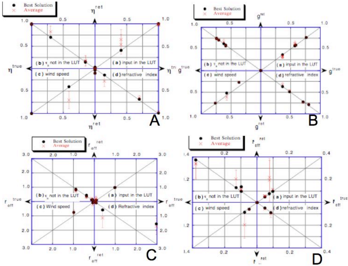
Figure 5: Same as Fig 4 but for (A) ratio \eta , (B) asymmetry parameter g , (C) Effective Radius ( R_{\text{eff}} ) and for (D) blowup of Effective Radius ( R_{\text{eff}} < 0.40 ). Error bars correspond to the standard deviation of the 'average' solution.
