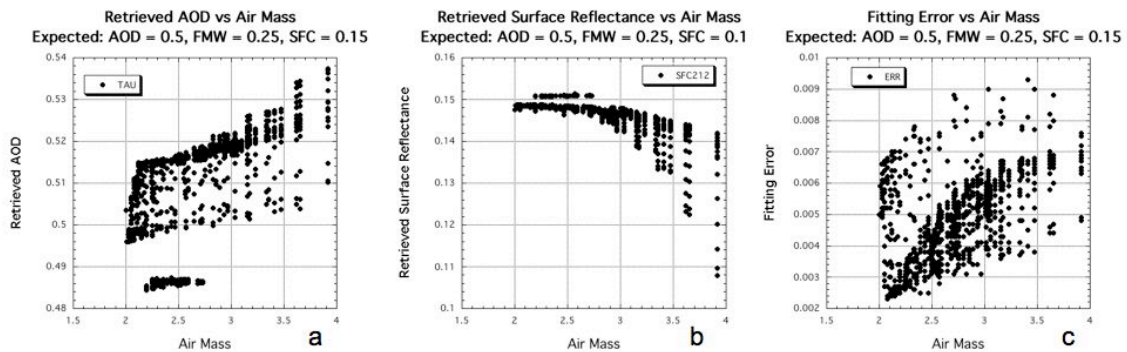
Figure 24: Retrieved MODIS products as a function of Air Mass for given atmospheric conditions ( \tau=0.5 , \eta=0.25 and \rho_{2.12}^s=0.15 ) and 720 LUT geometrical combinations. The retrieved AOD is plotted in (a) the 2.12 \mu\text{m} surface reflectance in (b) and the fitting error is plotted in (c). Note that in all cases, the FMW value of 0.25 was retrieved exactly. errors are much larger (up to 1%), but AOD is still well within expected error.
