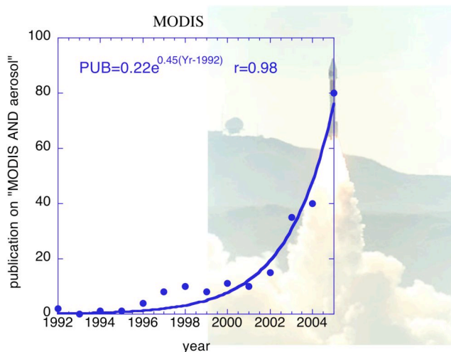
Figure 1: The image shows the exponential rate of publication from the ISI citation web site on "MODIS and aerosol" starting around 1992. (In the background is a photograph of the Terra launch on December 18, 1999). Operational algorithms and data centers that make the data available quickly to the broad international science community, give rise to an exponential publication rate preparing for and using MODIS aerosol data (Image produced by Y. Kaufman (climate.gsfc.nasa.gov)).
