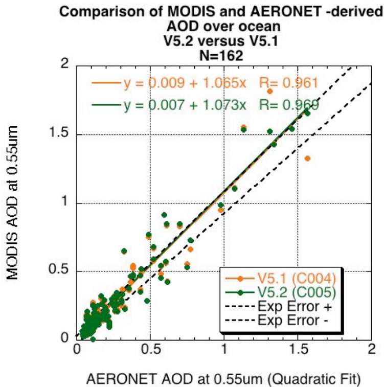
Figure 32: MODIS AOD over ocean retrieved at 0.55 \mu\text{m} , compared with AERONET AOD interpolated to 0.55 \mu\text{m} . Both the retrievals from V5.1 (orange) and V5.2 (green) are shown. The regressions (solid lines) are shown. The expected errors for MODIS ( \pm 0.03 \pm 0.05\tau ) are also shown (dashed lines).
