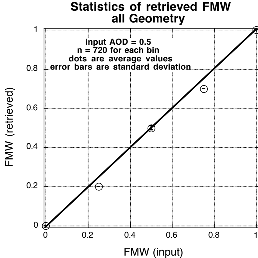
Figure 22: Scatter diagram of the retrieved FMW versus the input FMW. The open shapes correspond to the average of the solutions for each inputted FMW, where there are 720 combinations of geometry and input AOD. The error bars are the standard deviation of the 720 inputs. Only the FMW values of 0.0 and 1.0 would be represented exactly in the LUT, as all coarse and all fine model, respectively. Note the cases for which input FMW = 0.25 and FMW = 0.75, where the algorithm is only allowed to determine FMW in 0.10 increments.
