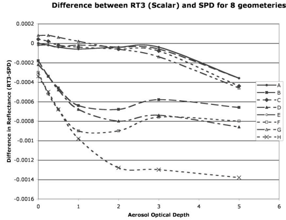
Figure 14: Difference between MIEV/RT3 combination and SPD derived reflectance at 0.466 \mu\text{m} , for eight example sun/surface/satellite geometries as a function of the input AOD.
