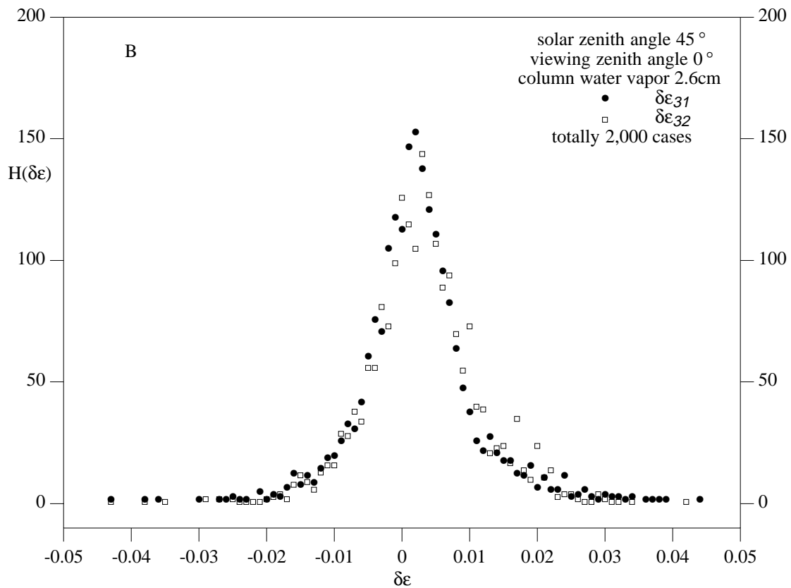
Figure 7, Histogram of errors in surface temperatures (A) and emissivities (B) retrieved by the \chi^2 fit method.
