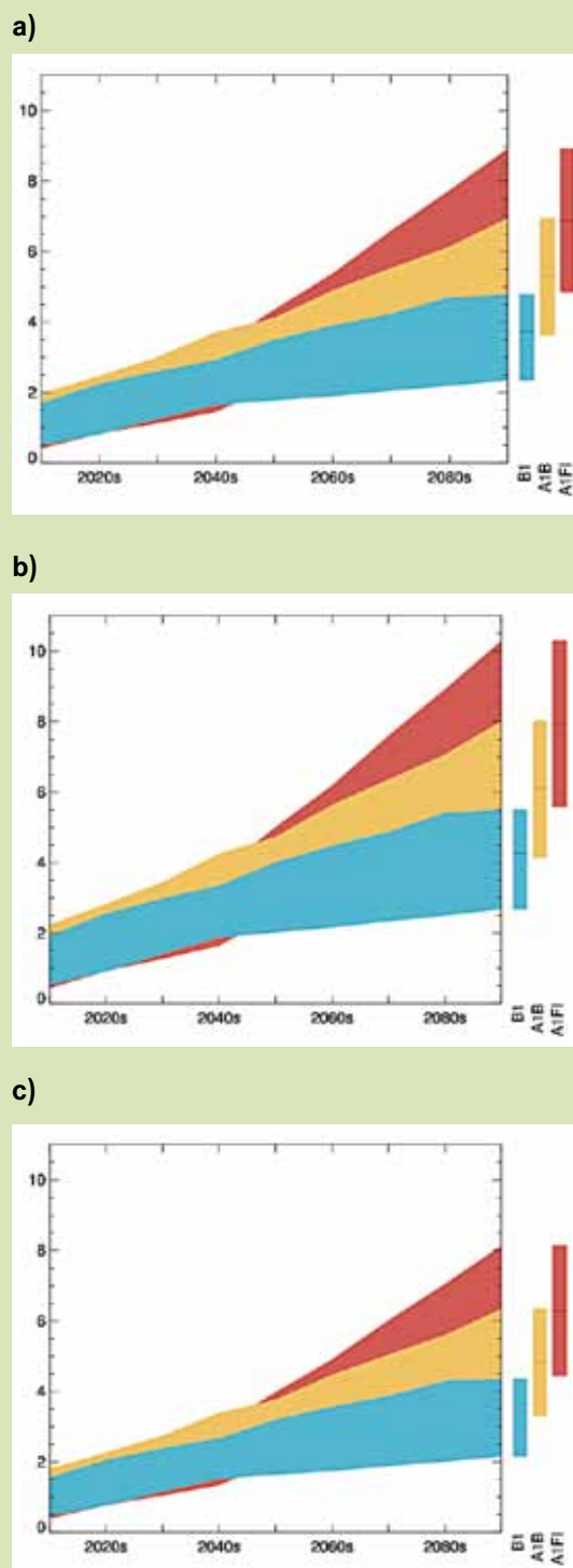
Figure 15: Projected change in a) annual average temperature (°C), b) average daily maximum temperature and c) average daily minimum temperature in the Amazon river basin over the 21 st century expressed relative to the 1961-90 baseline. The blue plume shows the range given by the 17 models of the low (B1) emissions scenario ensemble, the orange plume shows the medium (A1B) emissions scenario and the red plume shows the high (A1FI) emissions scenario. The bars at the side represent the range in uncertainty at the end of the 21 st century, with the darker horizontal line indicating the ensemble average value.
