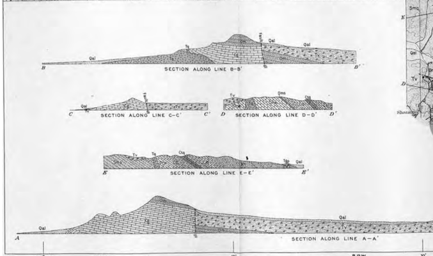
GEOLOGIC MAP AND SECTIONS OF THE MINING DISTRICTS OF THE H. B. Marshall, Chief Geographer; E. M. Douglas and T. G. Gardine, Geographers in charge Topography by W. M. Beaman and Fred McLaughlin Control by Coast and Geodetic Survey and Fred McLaughlin. Surveyed in 1904-1908 and 1909. Scale 42800 Contour interval 50 feet. Datum is mean sea level. Assuming elevation of Price derived from railroad level. 1903
