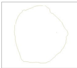
Figure 12b. Southern Hemisphere Median Shapefile for month of April, 1981 - 2010.
