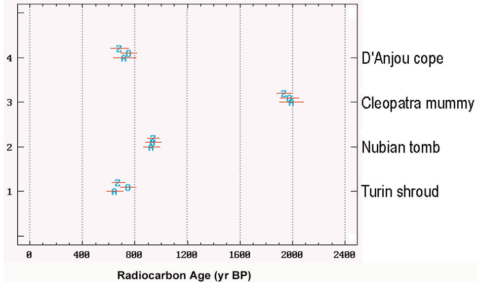
Fig. 16. AMS 14 C dating results (“blind”) for the Turin Shroud (sample-1) and three control samples of known age (samples-2,3,4), from the three AMS laboratories: Z (Zürich), O (Oxford), and A (Arizona). Dates are expressed as “Radiocarbon Years” before present (BP); uncertainties represent 95 % confidence intervals [38].
