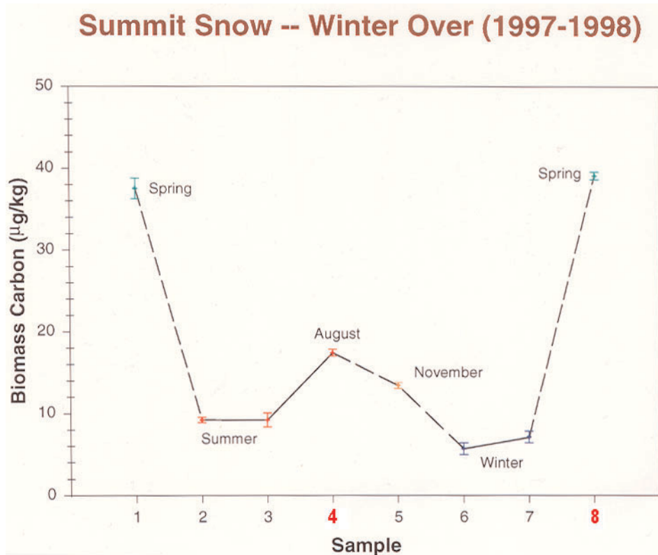
Fig. 21. First evidence of a seasonal pattern in biomass carbon aerosol in surface snow in central Greenland [55, 56]. Fundamental differences were found between the biomass carbon peaks in summer (sample-4 [WO4]), and spring (sample-8 [WO8]) via “multi-spectroscopic” macro- and micro-chemical analysis.
