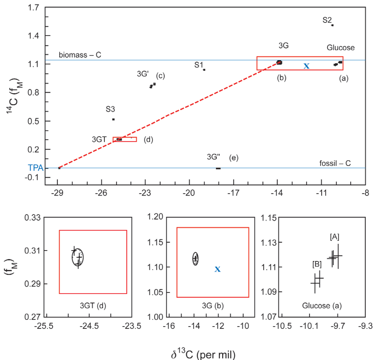
Fig. 10. Unique Isotopic Signatures: the ^{14}\text{C} - ^{13}\text{C} plane [25]. The main panel shows dual isotopic signatures f : for (1) NIST (S1, S3) and IAEA (S2) traceability standards, and (2) glucose from biomass (a), the new bio-sourced monomer 3G (b) (from cornstarch), the resulting copolymer 3GT (d), and pre-existing products 3G', 3G'' (c, e). Expanded views of the authentication regions (red rectangles) for the copolymer (left) and monomer (center) are given in the bottom panels, plus \approx 10 -fold expansion (right) of the isotopic data for independent batches (A, B) of a biomass feedstock (glucose from corn). The blue "x" represents a blind (3G) validation sample.
