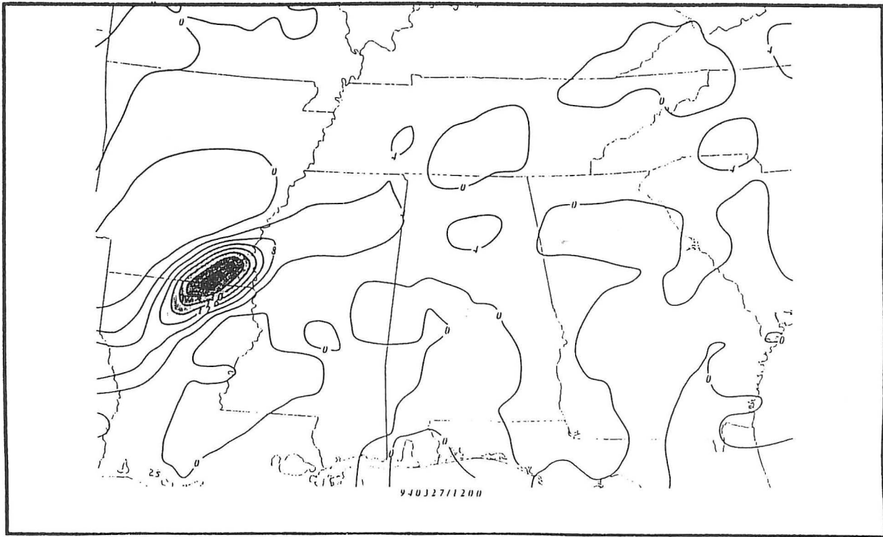
Fig. 8. Surface frontogenesis ( \Theta 100 \text{ km}^2 3 \text{ h}^{-1} ) from Langmaid et al. (1996).
