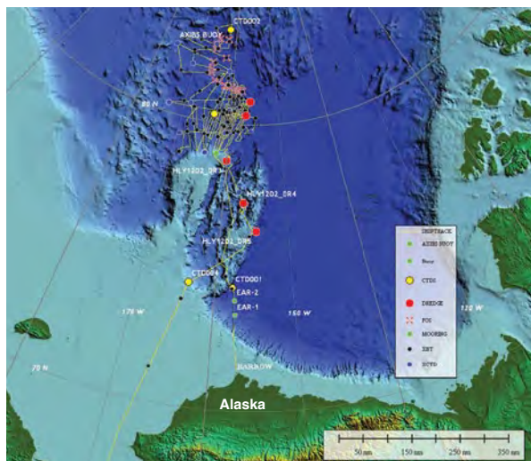
Tracklines for 2012 Arctic ECS cruise aboard USCGC Healy focused on the region north of Barrow, AK, between the Nautilus Basin and the Alpha/Mendelev Ridge UNH/NOAA
