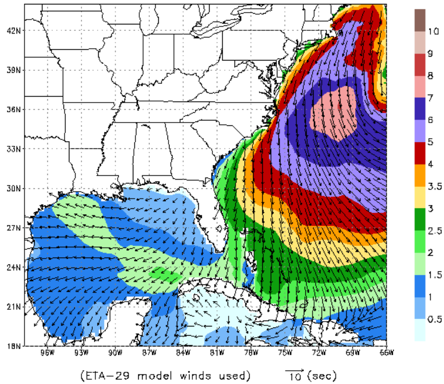
Fig. 5 An example of 24-hr forecast of wave pattern caused by Easter storm 1997.
