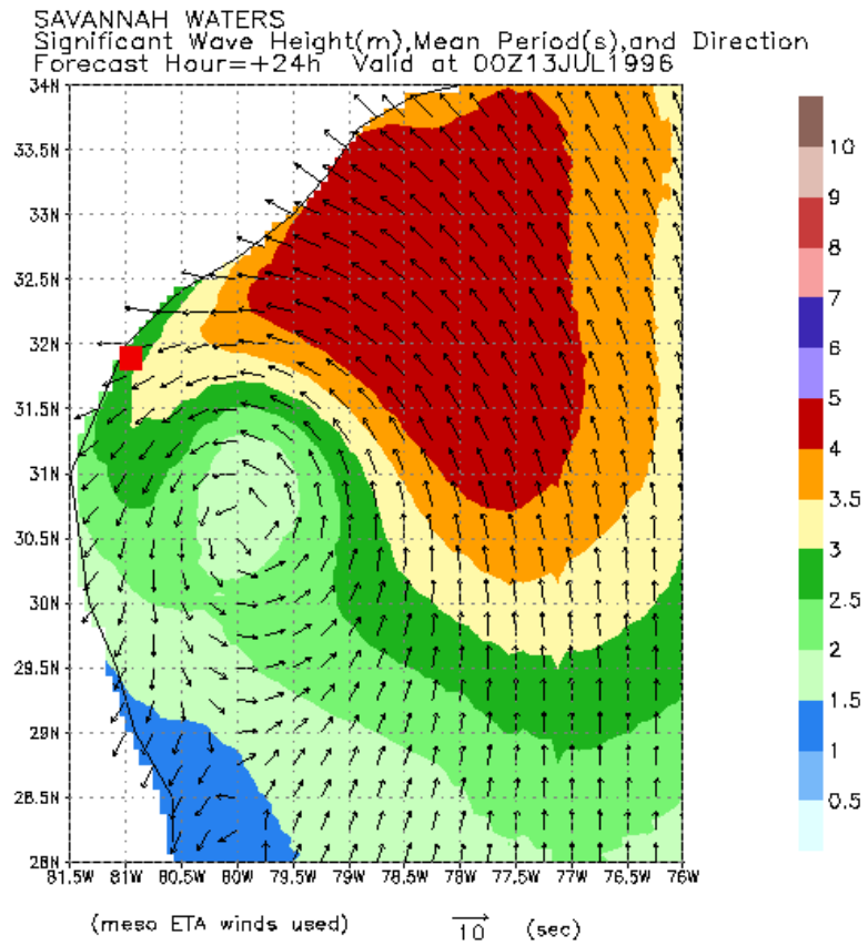
Fig. 3 An example of 24-hr forecast of wave pattern caused by Hurricane Bertha 1996.
